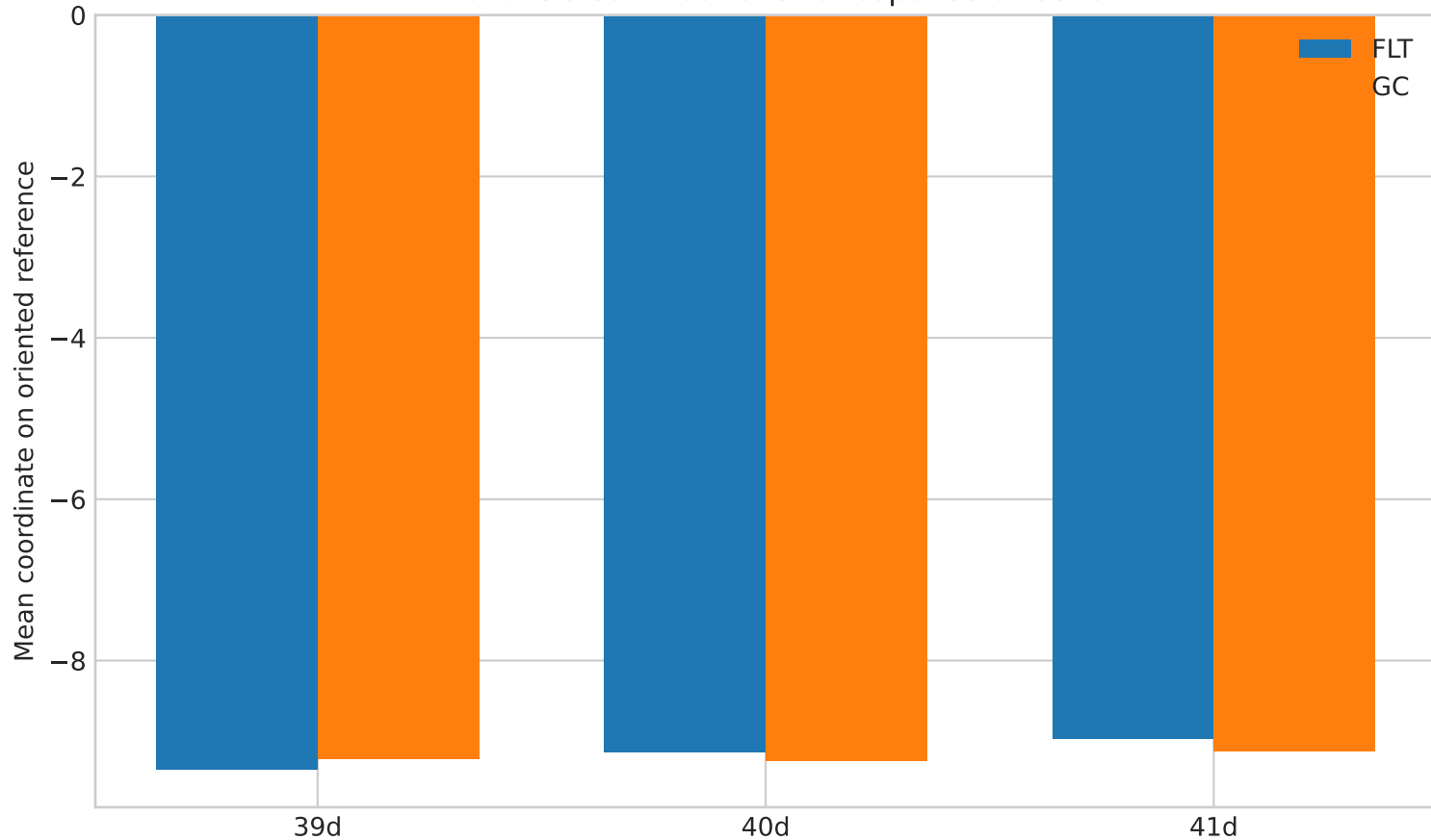
FLT and GC contributions to response direction
