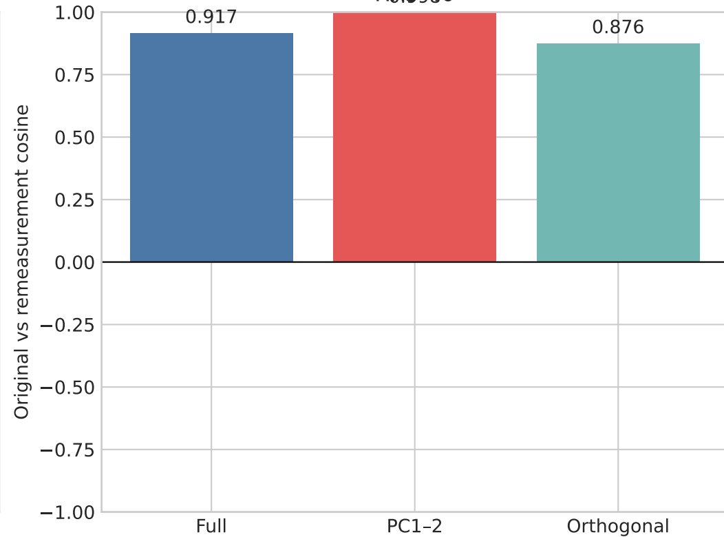
RR3 response replication by controlled-reference component
