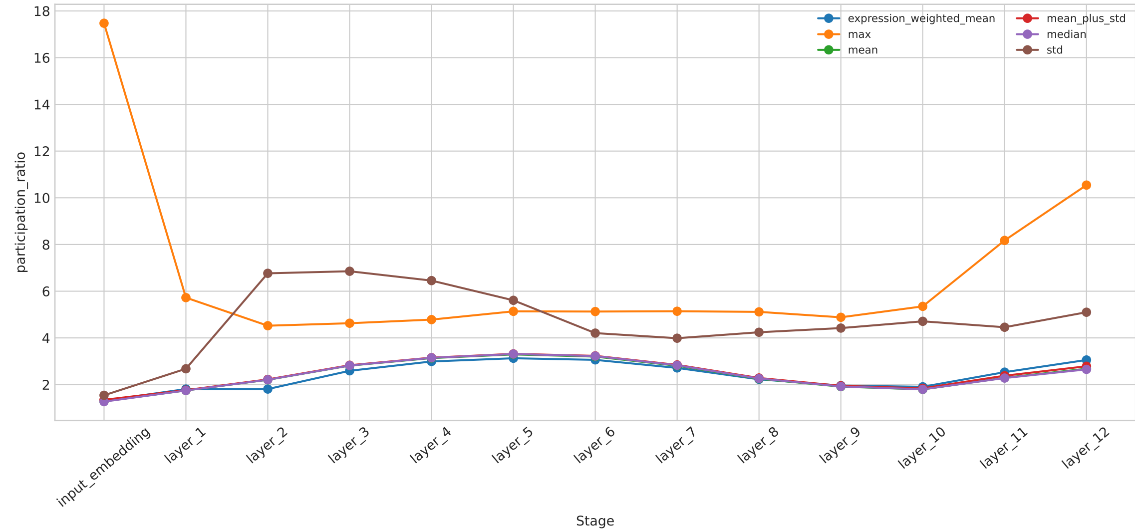
Effective dimensionality through BridgeRNA
