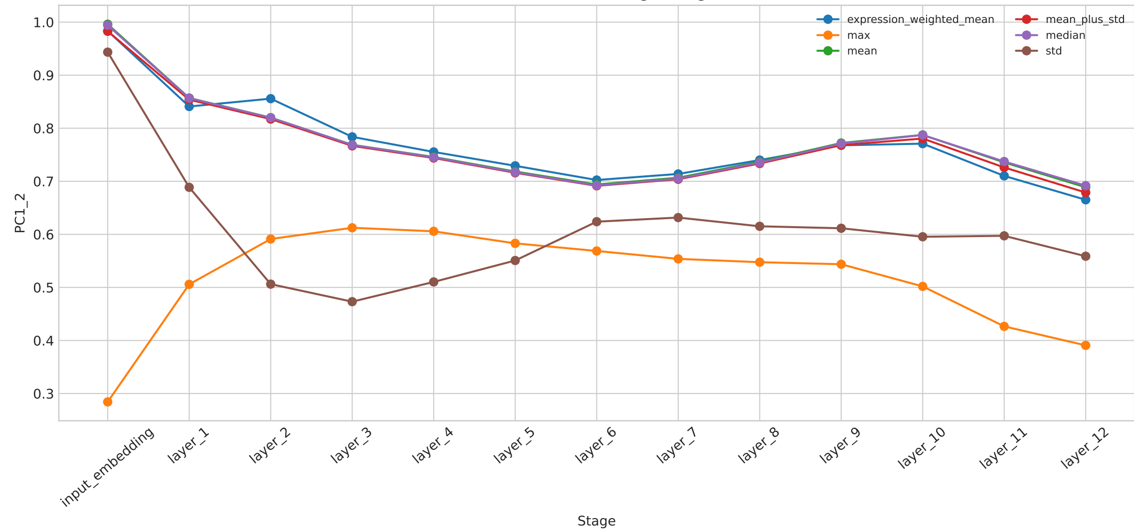
PC1+PC2 variance through BridgeRNA
