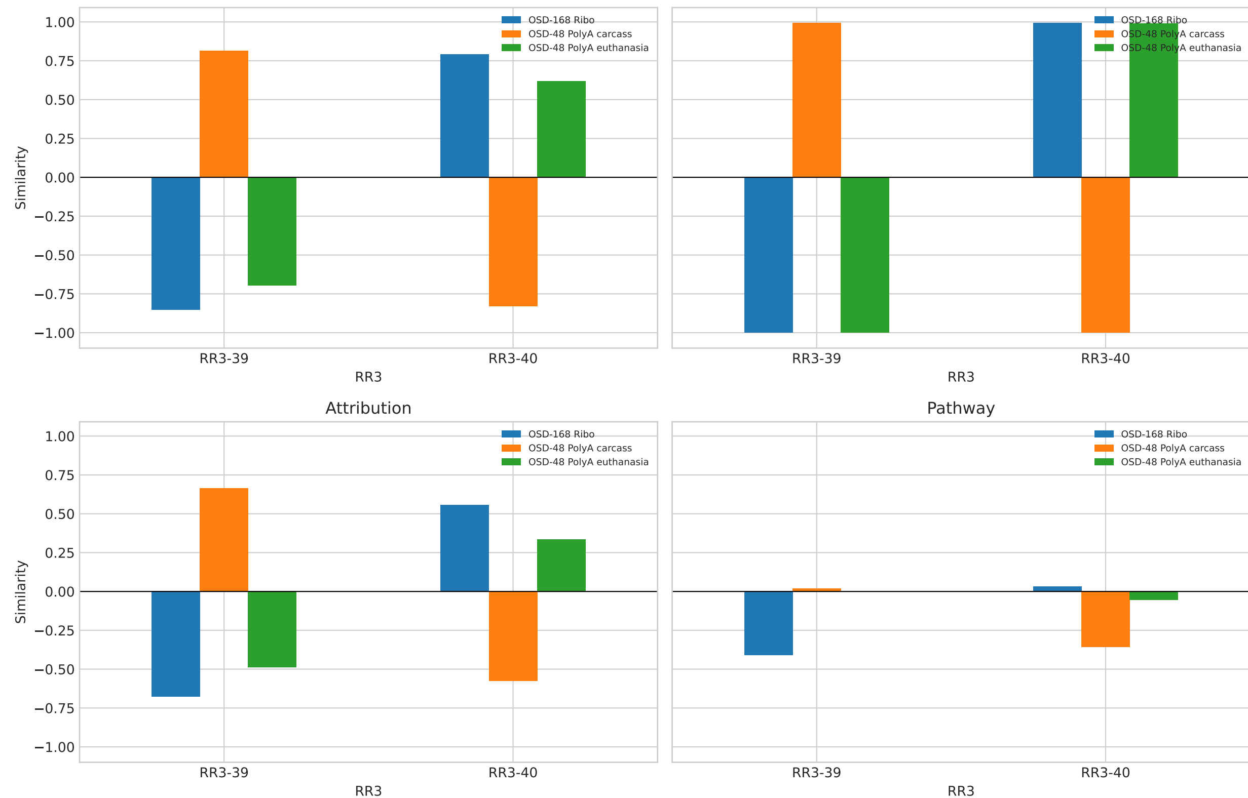
Full latent
