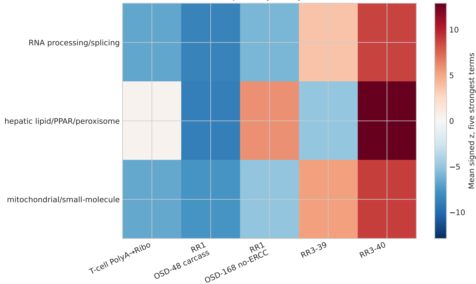
Measured pathway-family attribution
