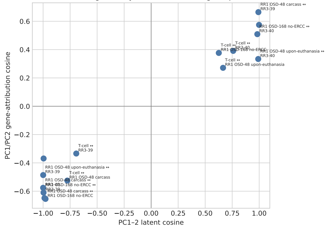
Same latent geometry can use different gene profiles
