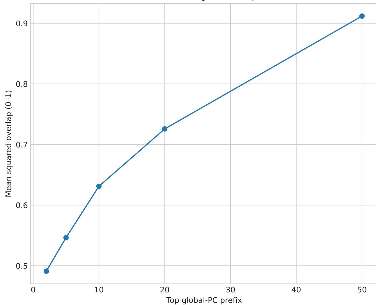
T-cell PC1-2 vs global-PC spaces
