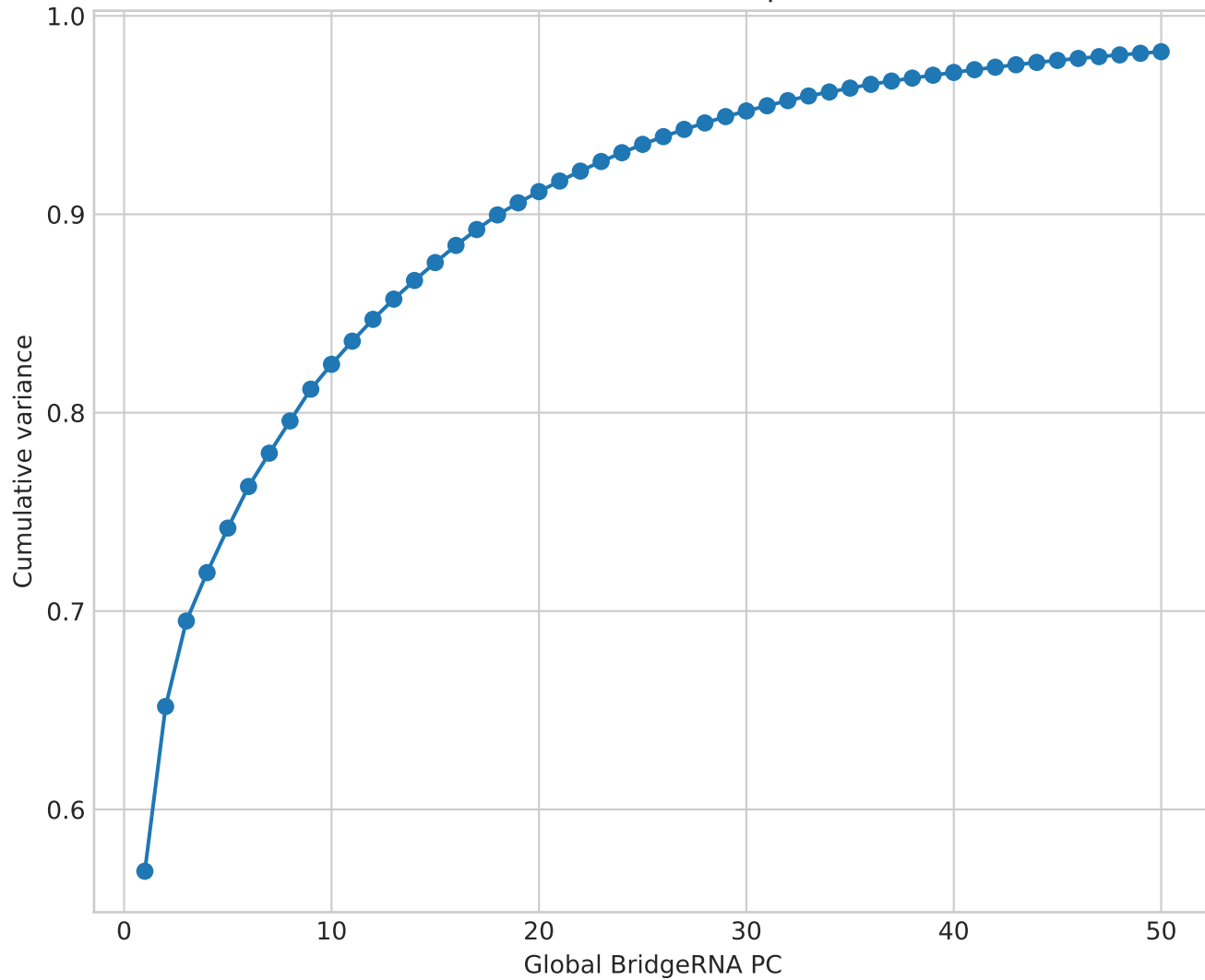
Global latent variance spectrum
