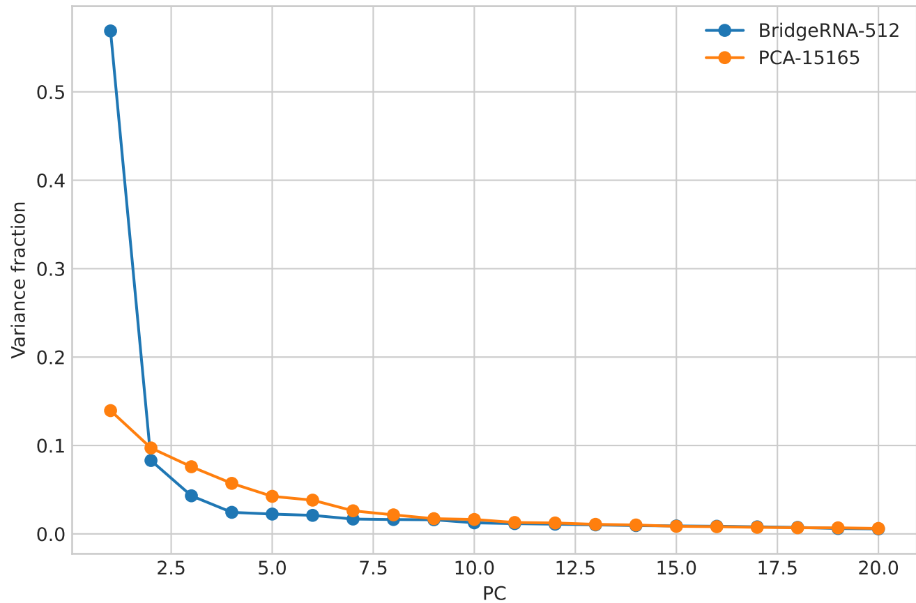
First 20 PCs
