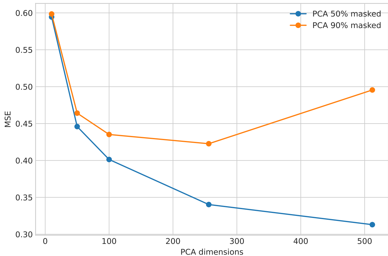
External TCGA masked reconstruction
