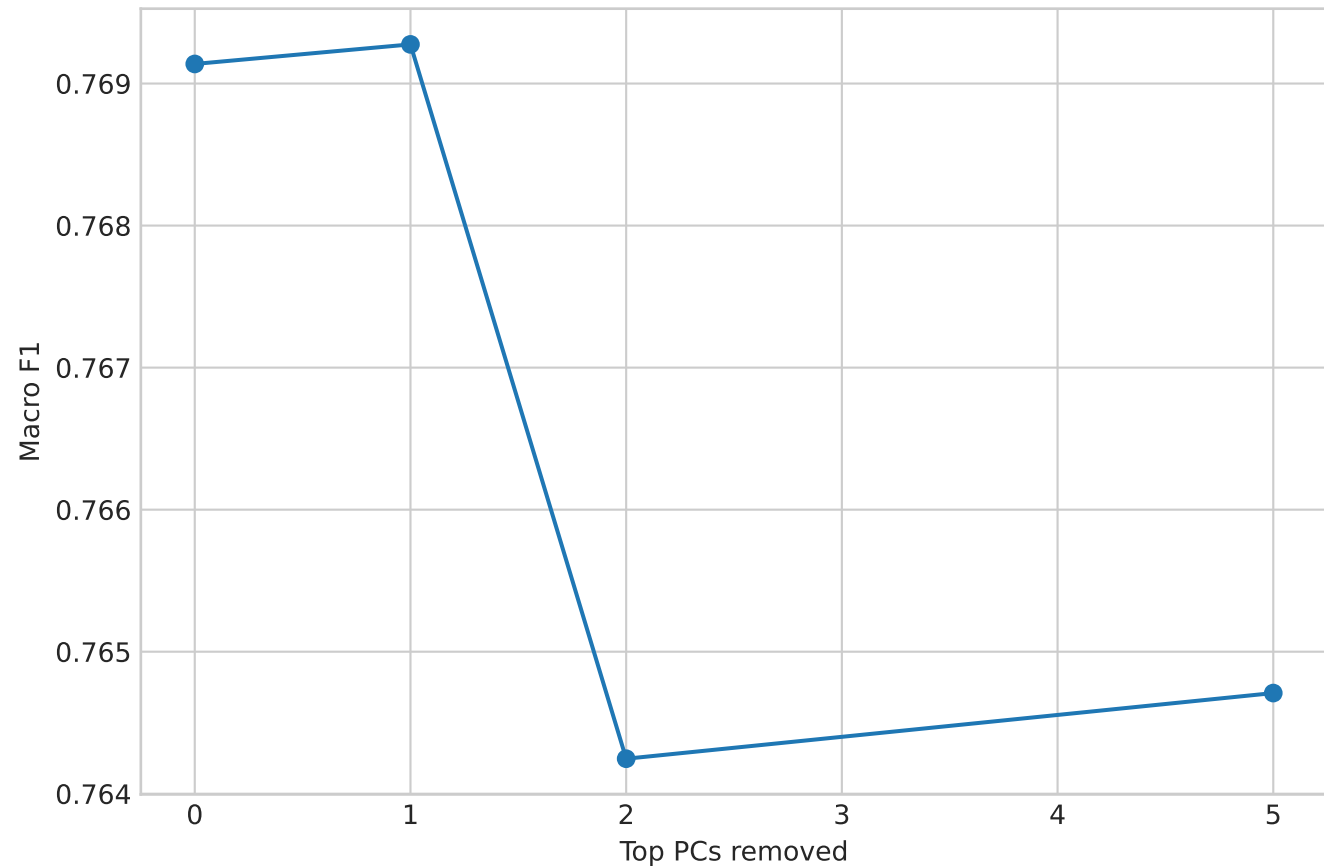
BridgeRNA dominant-PC sensitivity
