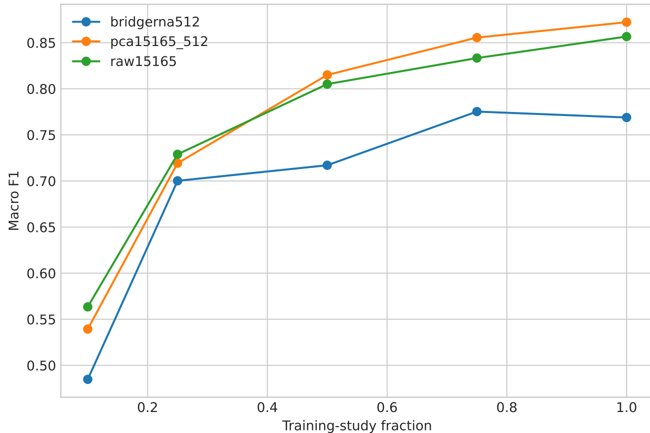
Low-label learning curve
