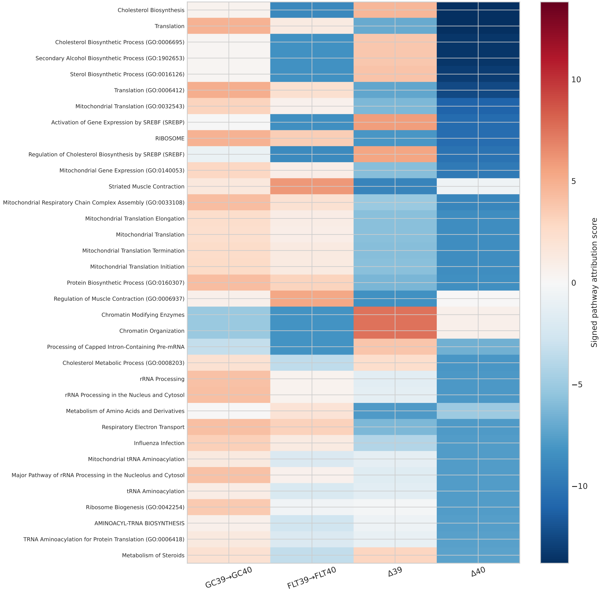
Four-state contextual pathway profiles
