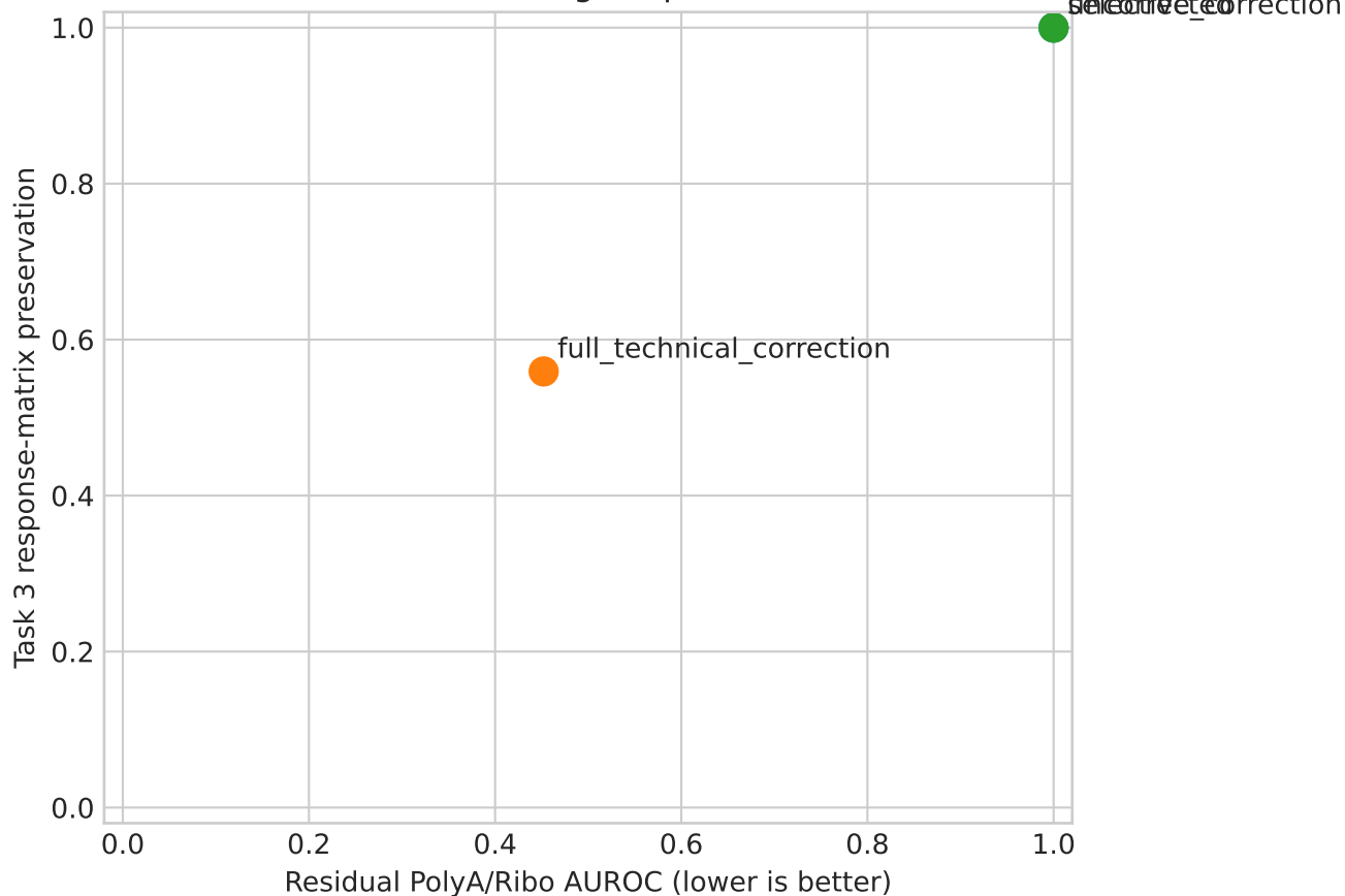
Technical-removal / biological-preservation tradeoff
