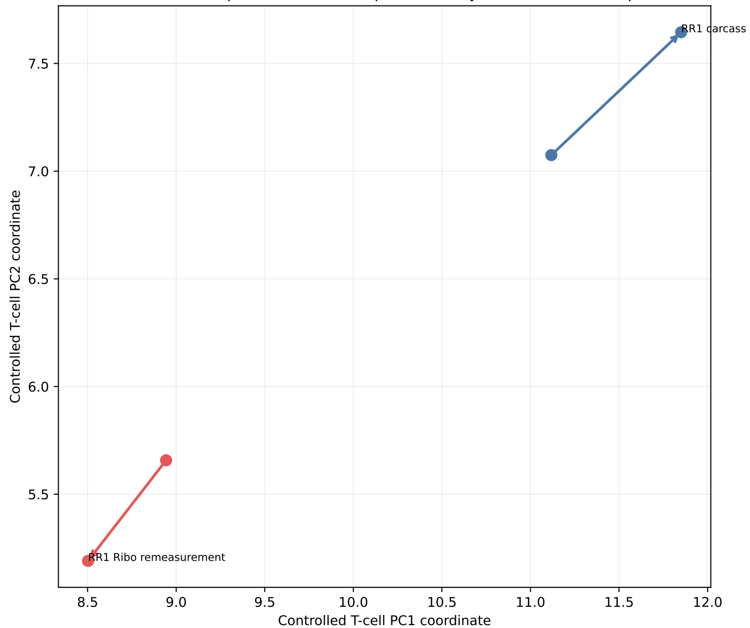
RR1 FLT–GC responses in the independent PolyA/Ribo-associated plane
