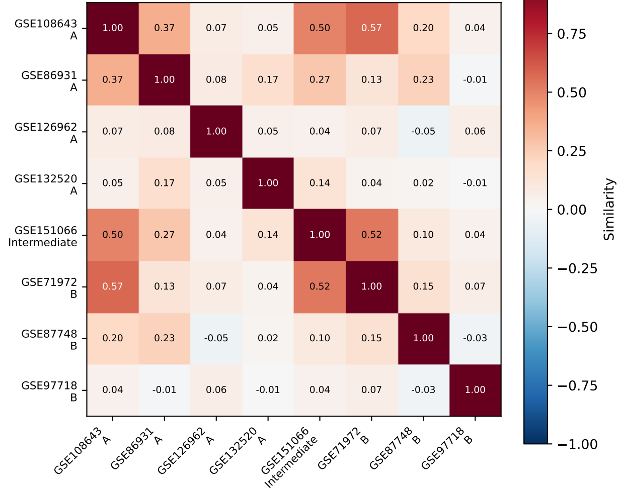
Spearman correlation
