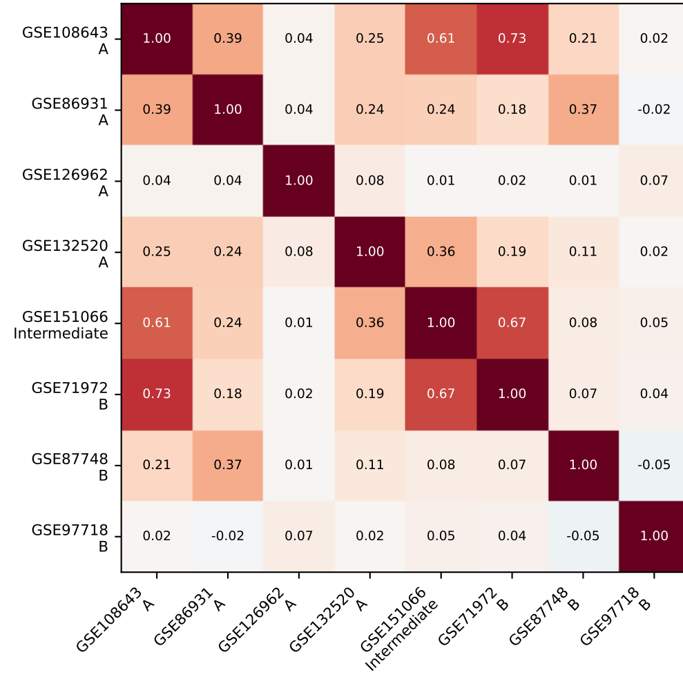
Cosine similarity
