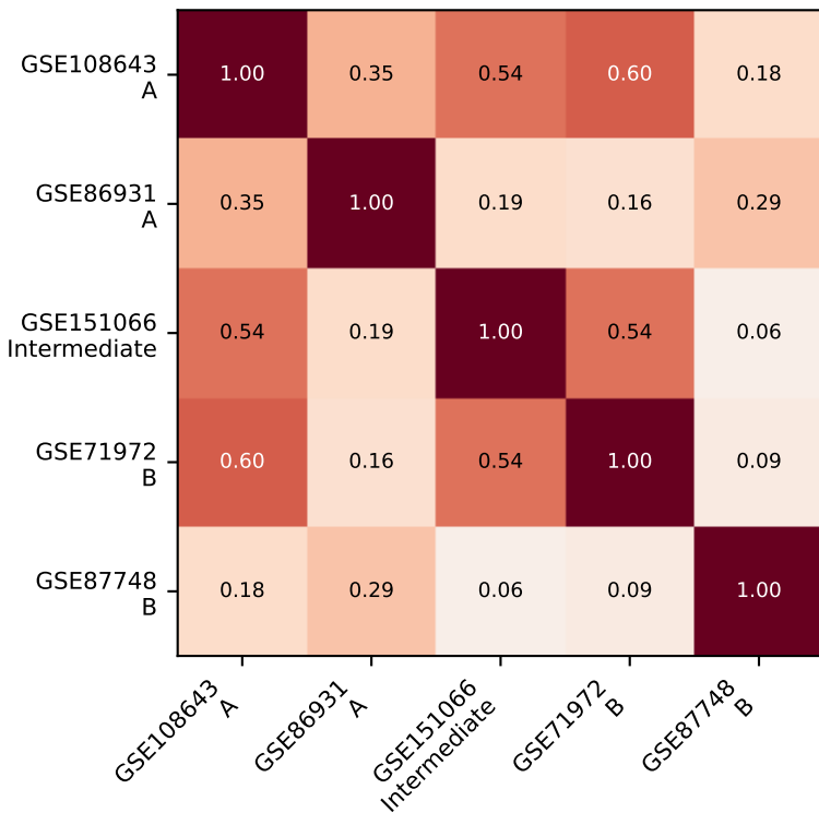
Cosine similarity
