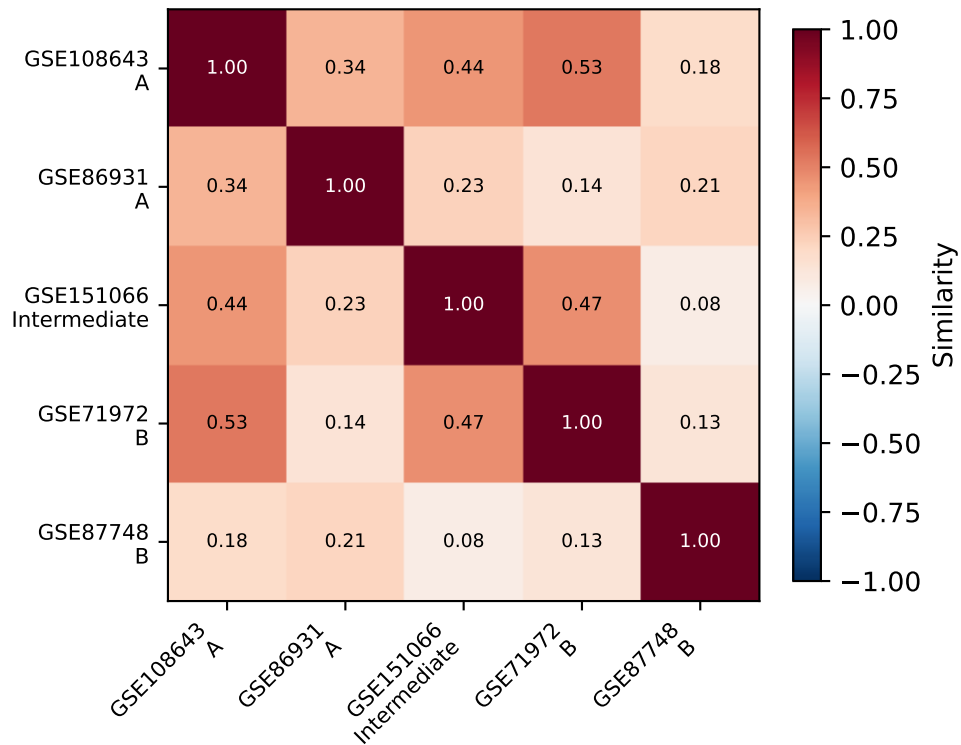
Spearman correlation
