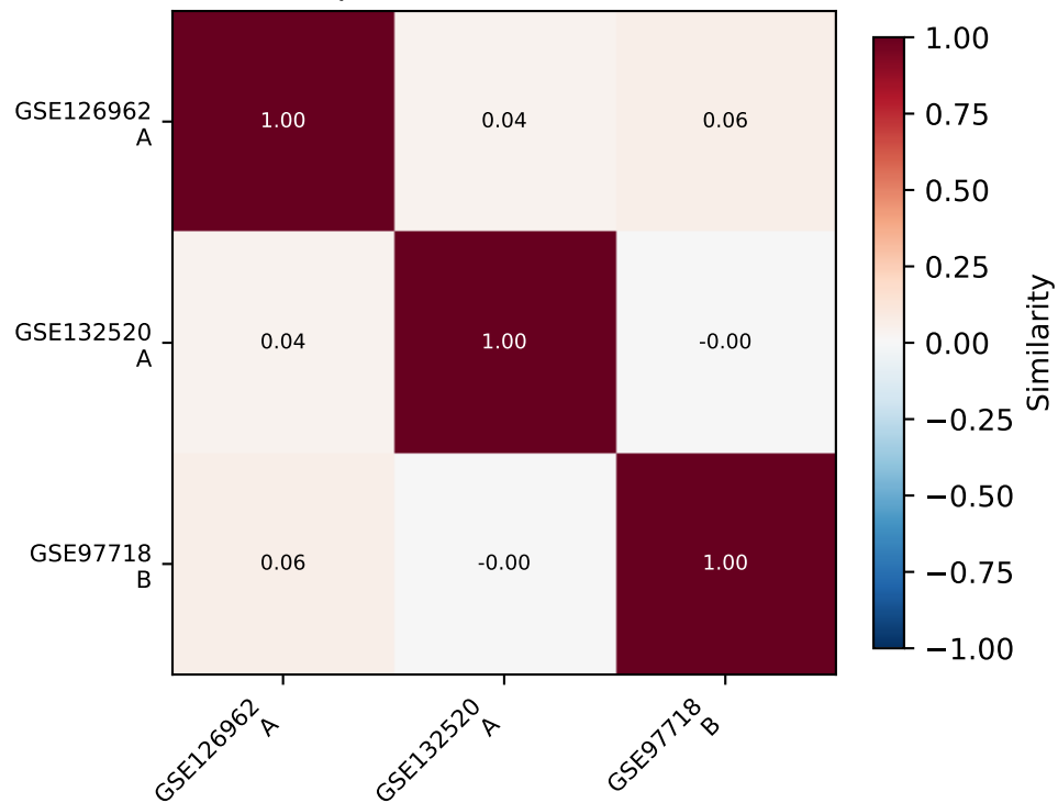
Spearman correlation
