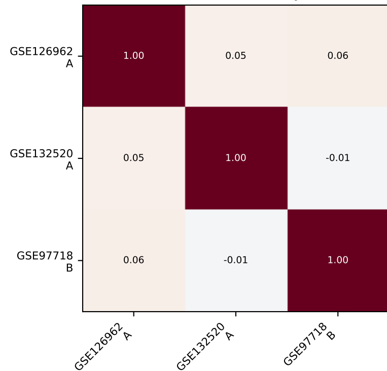
Cosine similarity
