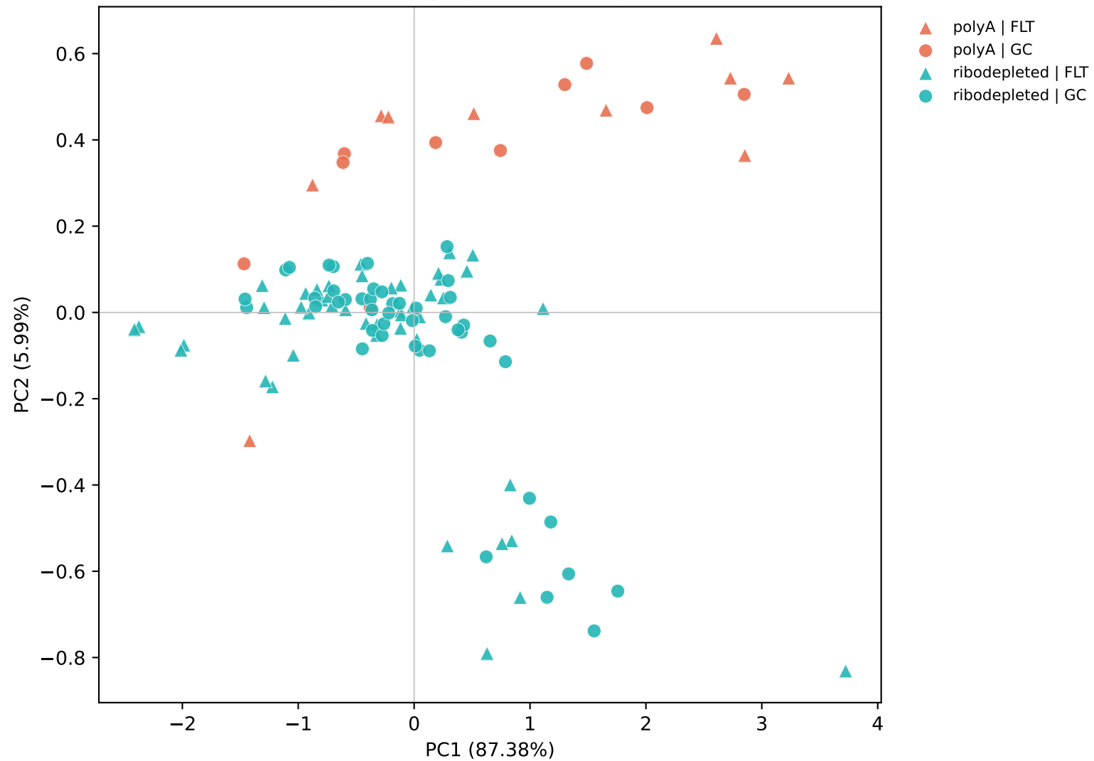
Frozen BridgeRNA embedding PCA colored by library preparation; shape = FLT/GC
