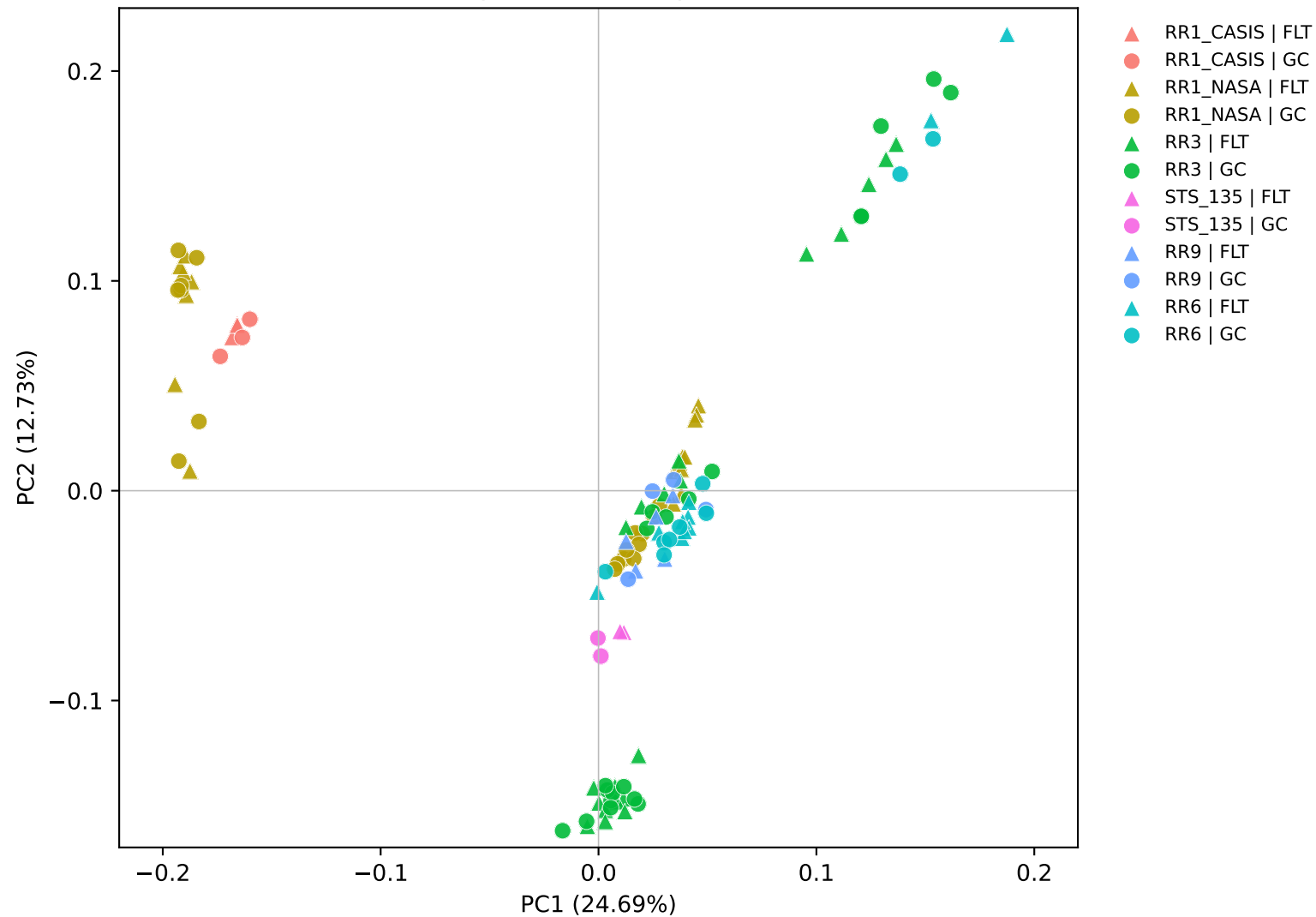
Sanders Figure 1 reproduction: \log_2(\text{DESeq2-normalized counts} + 1) colored by mission; shape = FLT/GC
