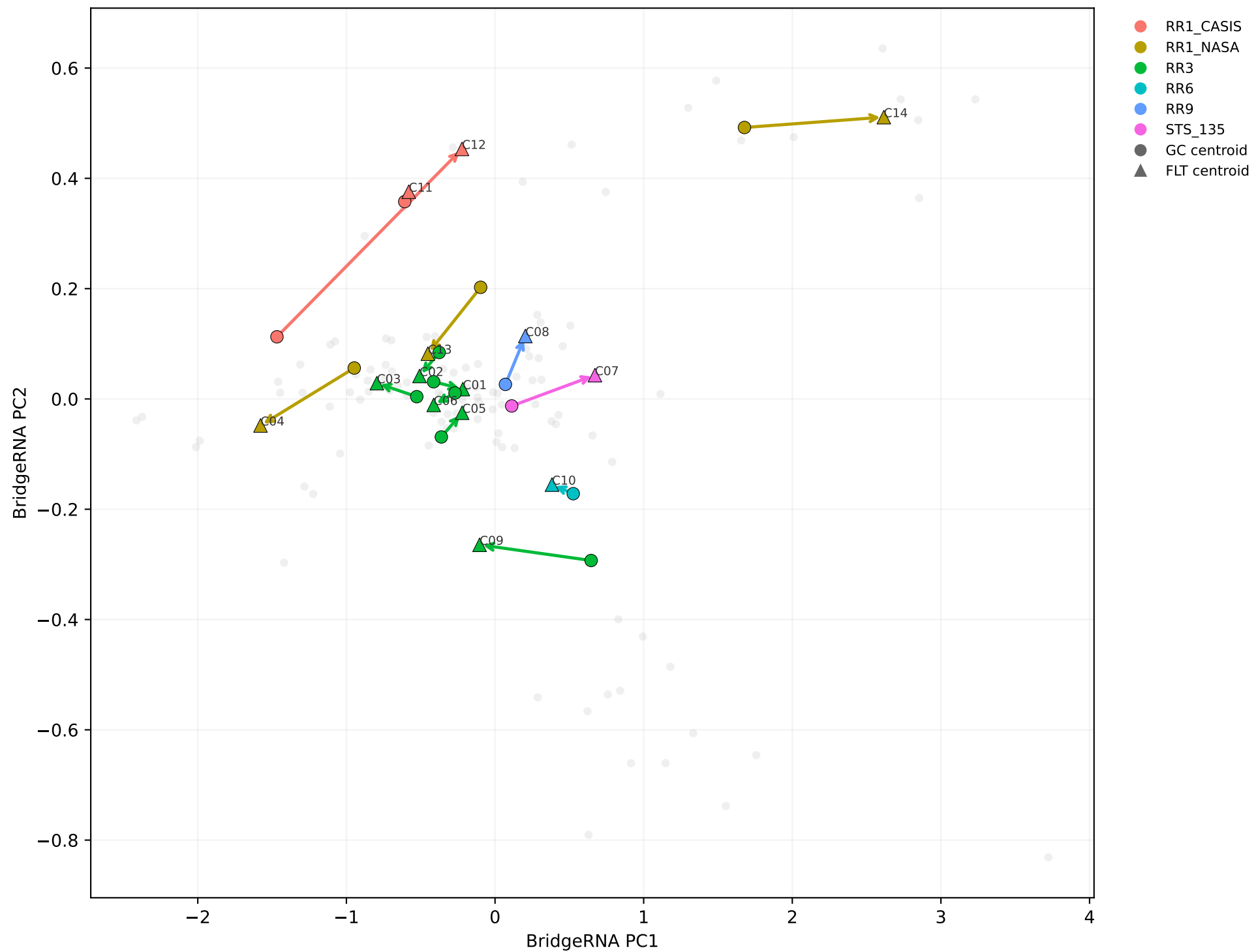
Within-stratum spaceflight displacement in frozen BridgeRNA space arrow: GC centroid → FLT centroid
