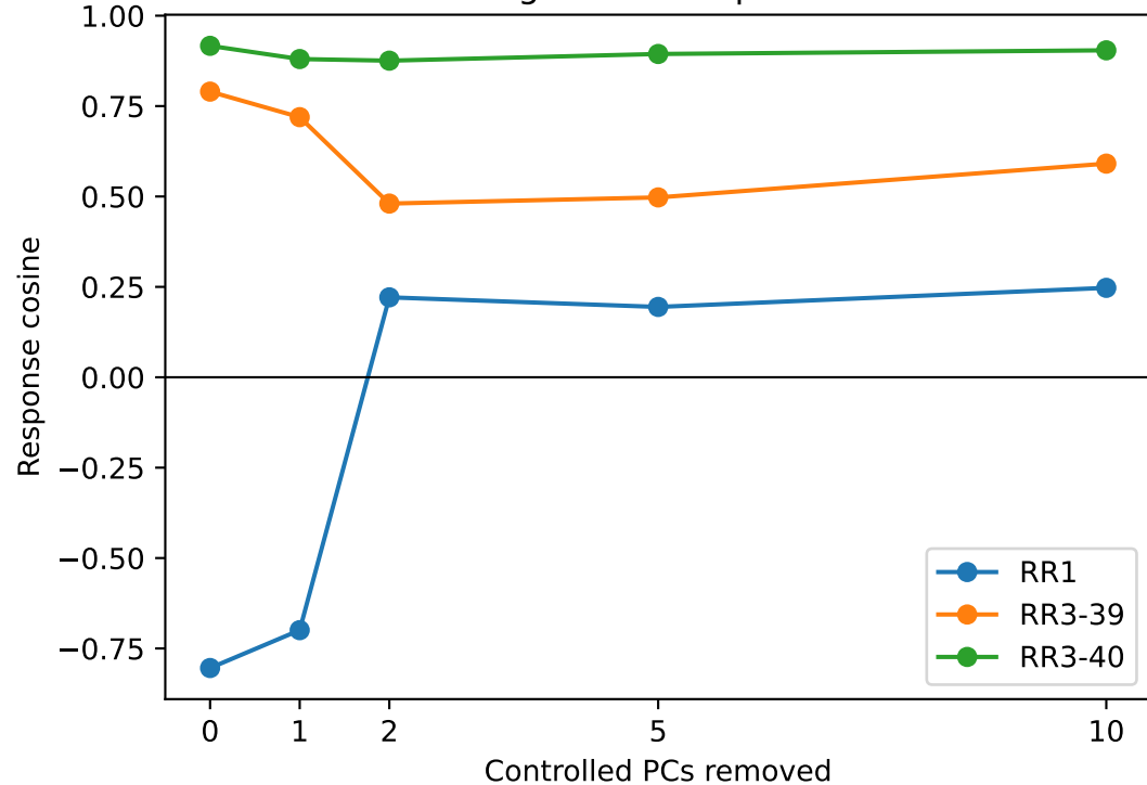
Task 3 diagnostic subspace removal
