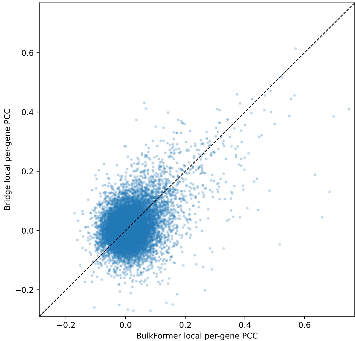
Matched genes (n=14,415)
