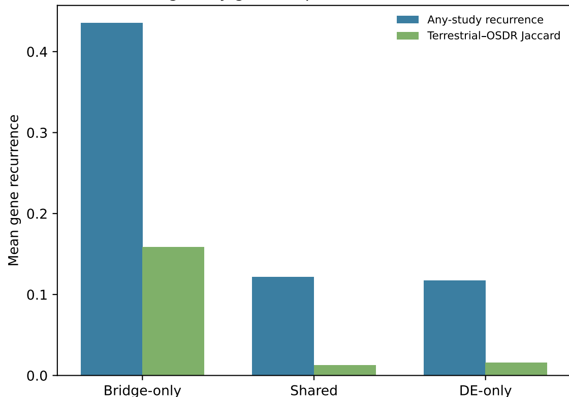
Bridge-only genes reproduce across studies
