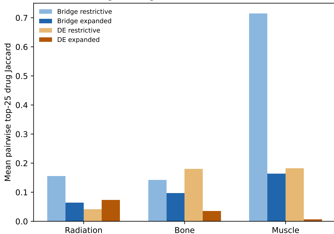
Drug convergence is resource-sensitive
