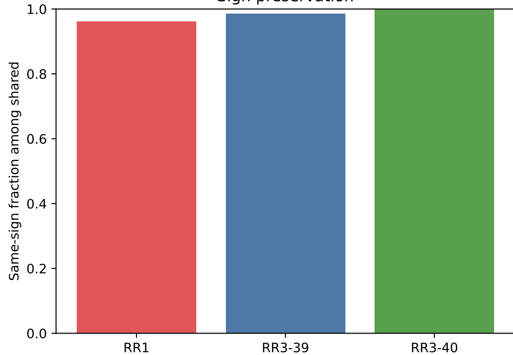
Sign preservation
