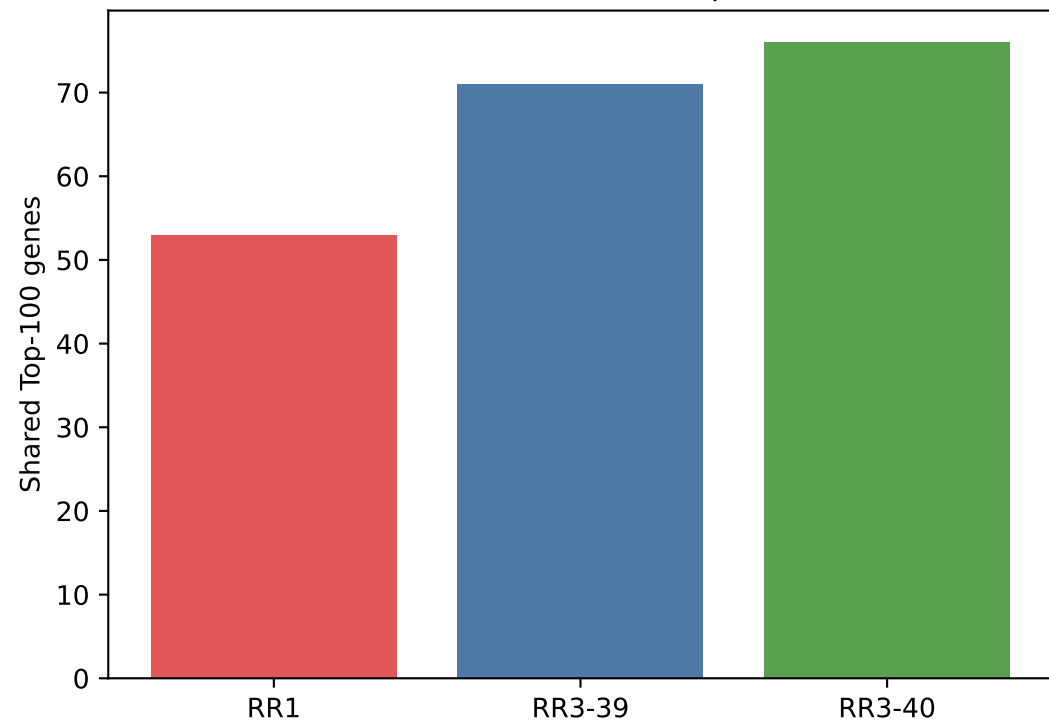
Attribution overlap
