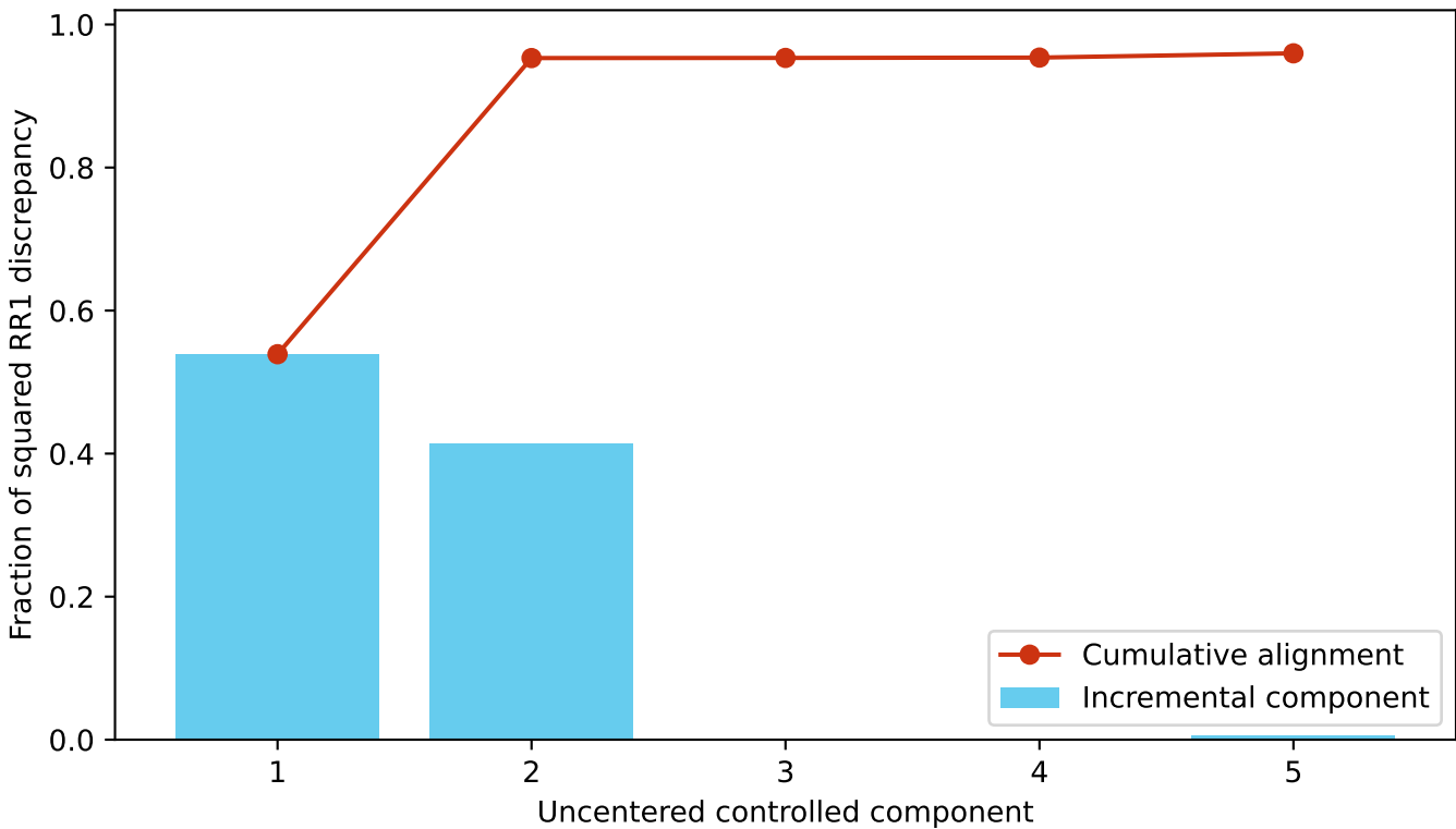
RR1 alignment beyond the dominant controlled direction
