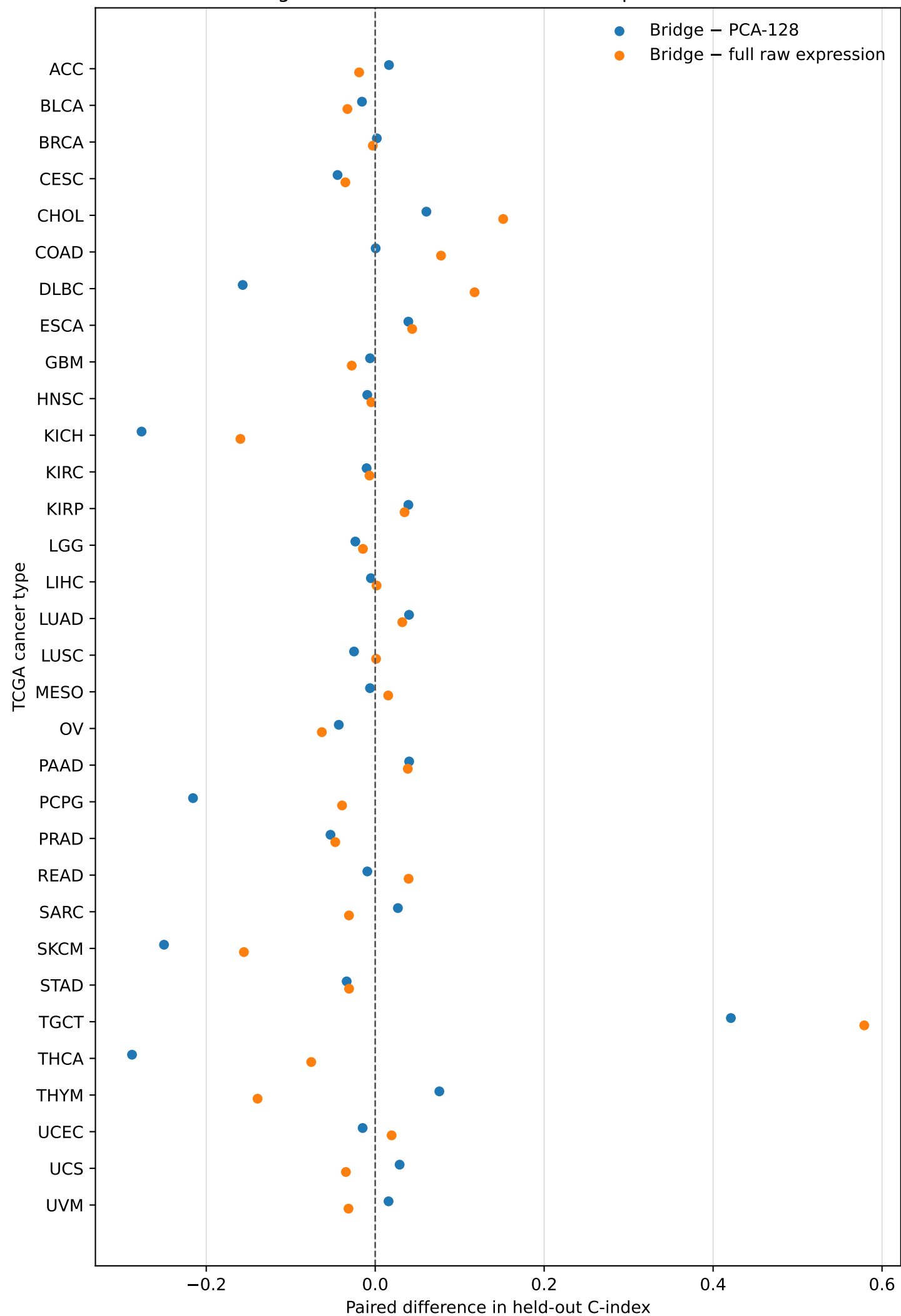
Bridge versus conventional survival representations
