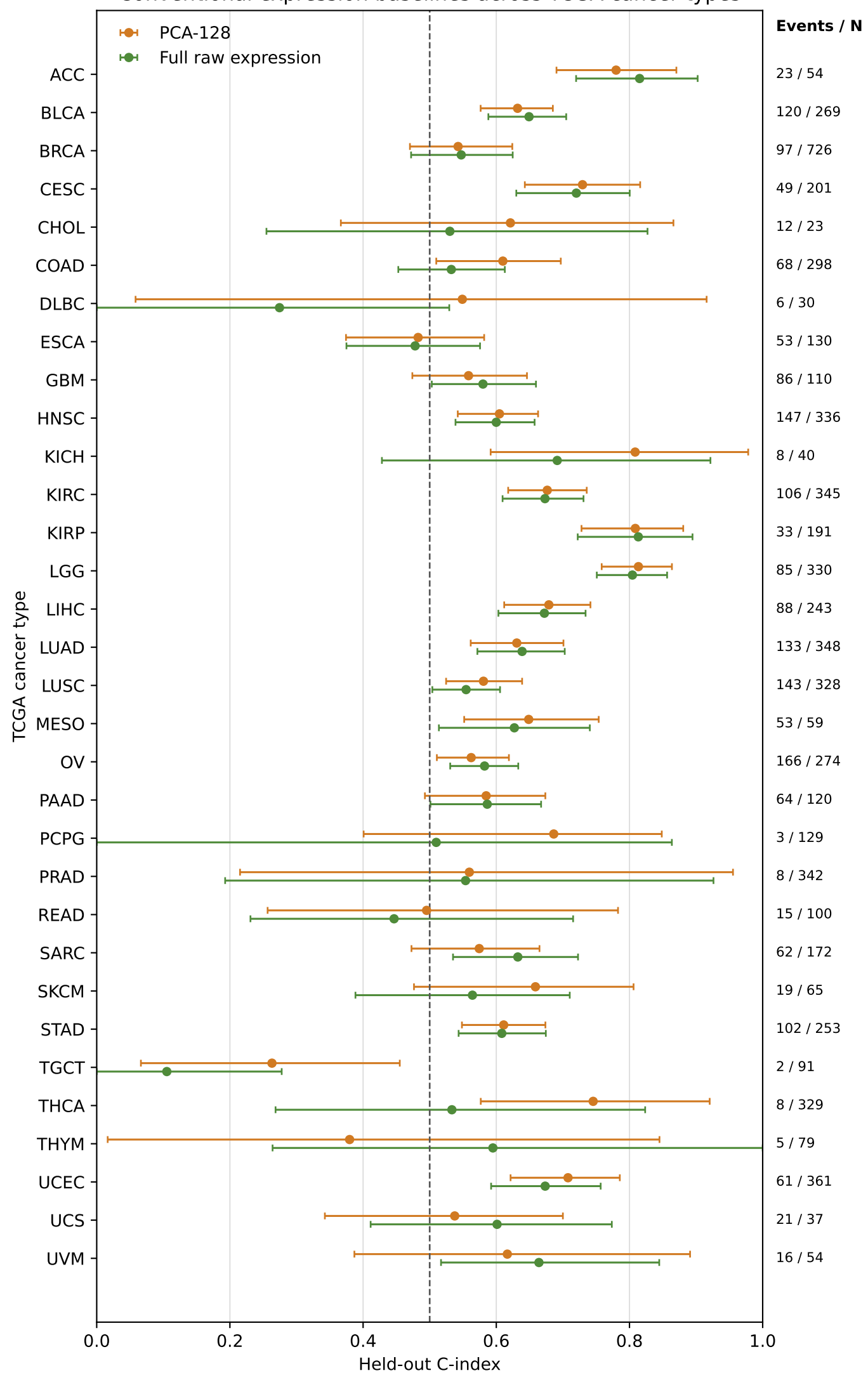
Conventional expression baselines across TCGA cancer types
