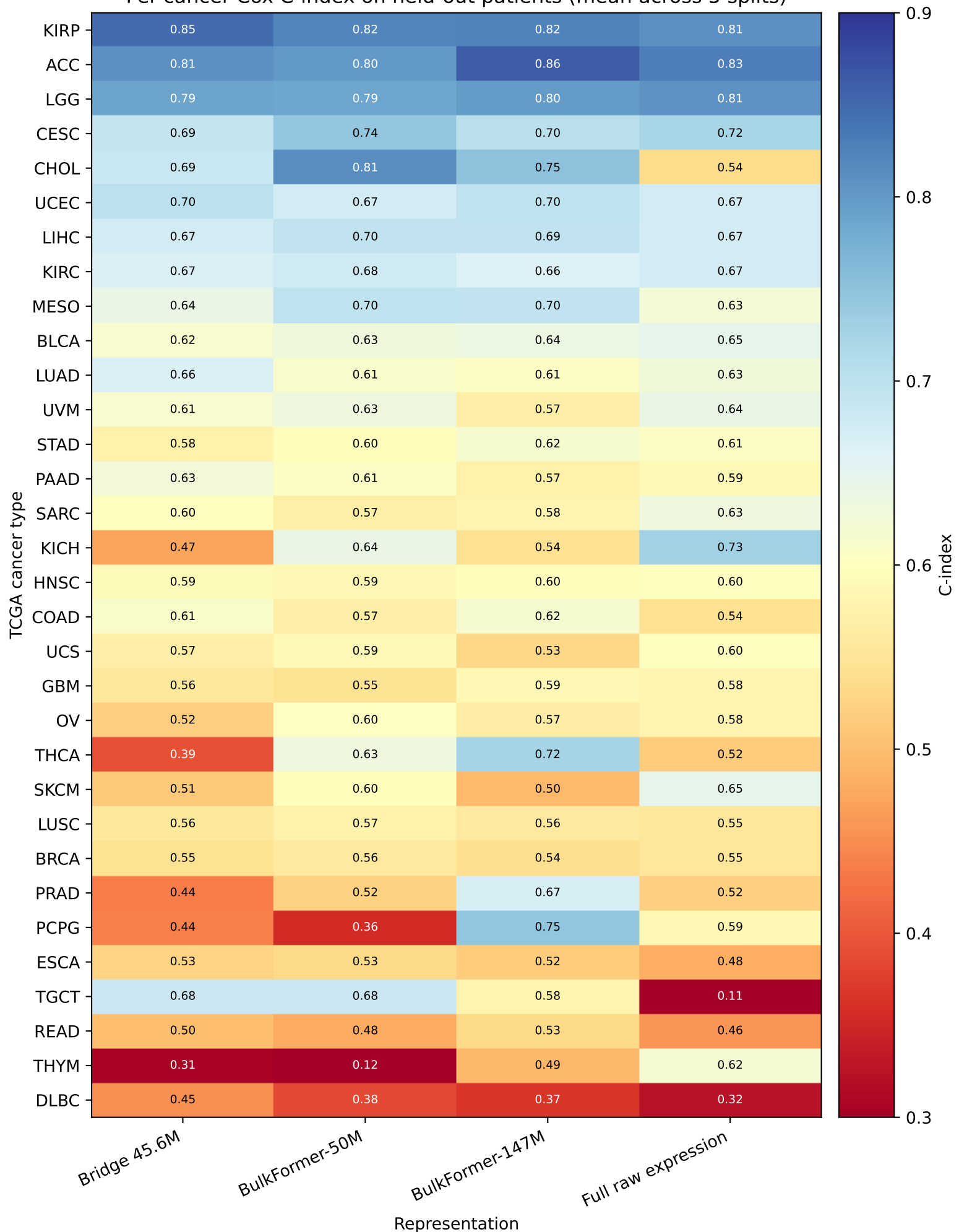
Per-cancer Cox C-index on held-out patients (mean across 5 splits)
