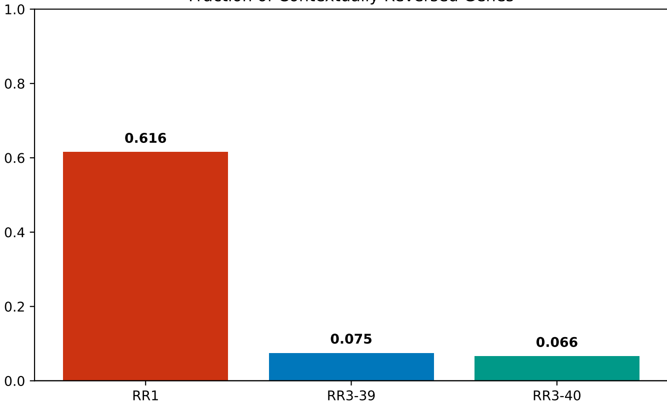
Fraction of Contextually Reversed Genes
