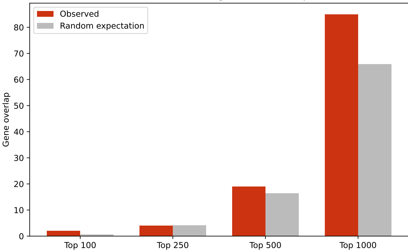
RR1 vs controlled gene-level overlap
