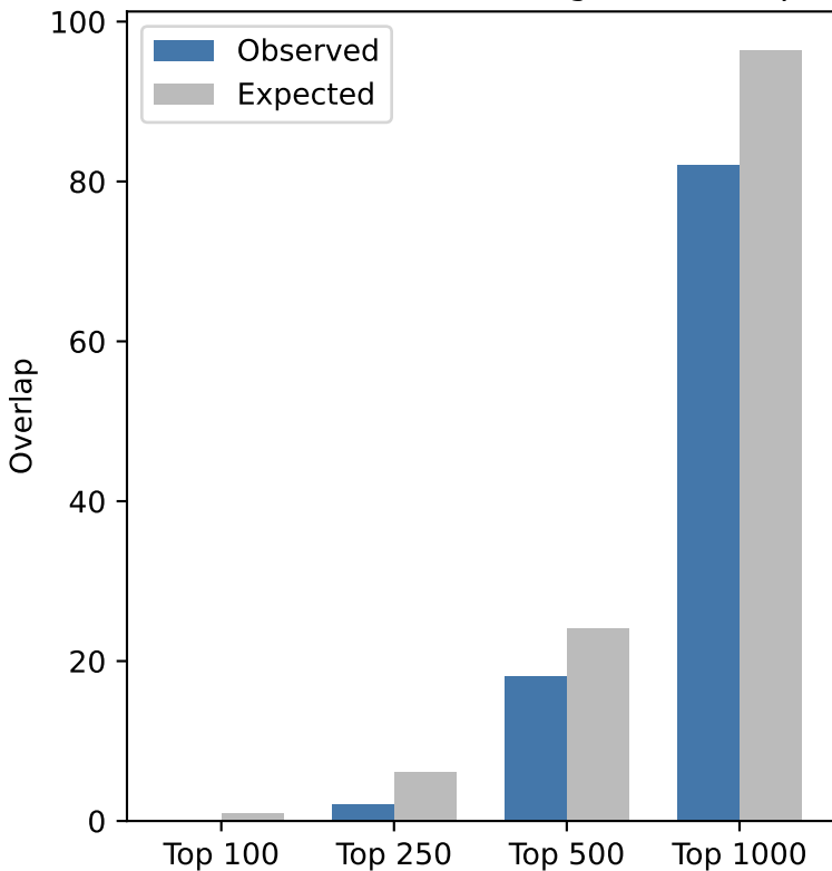
Cross-context residual gene overlap
