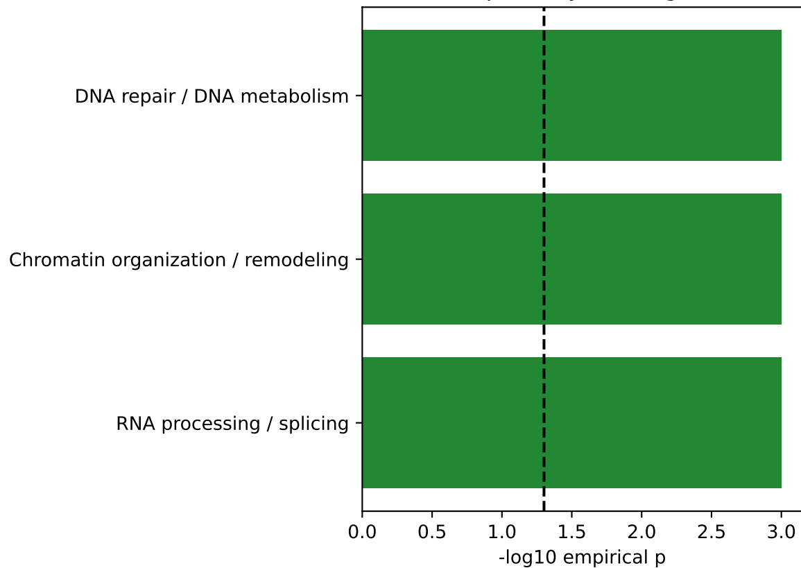
Residual pathway-convergence null
