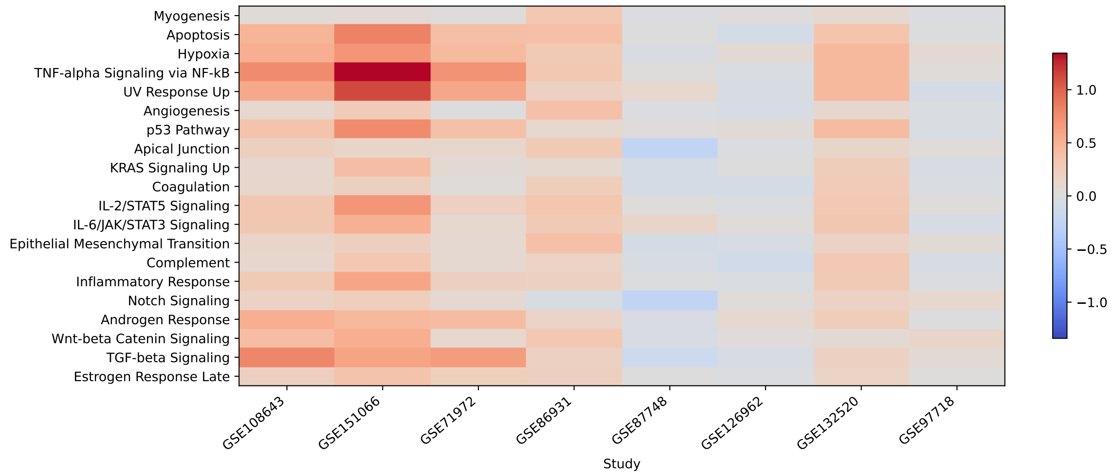
Direct ssGSEA Hallmark \Delta
