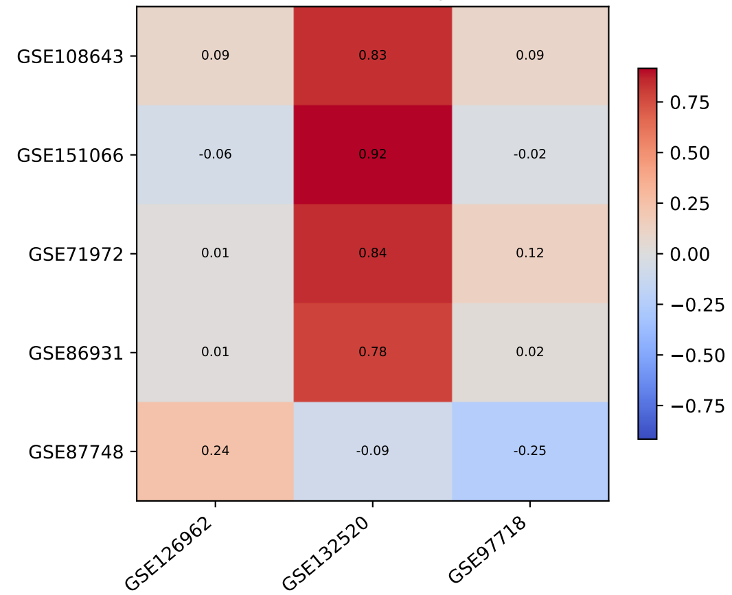
Direct ssGSEA response
