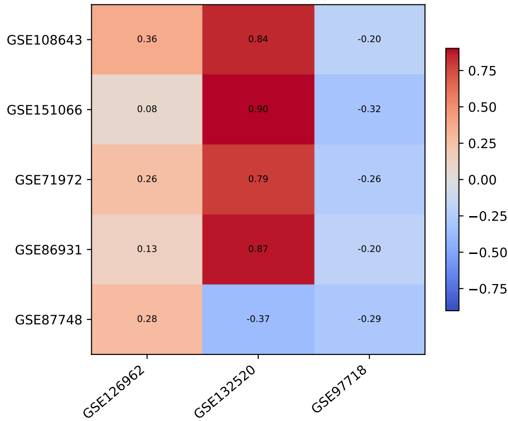
Predicted Hallmark response
