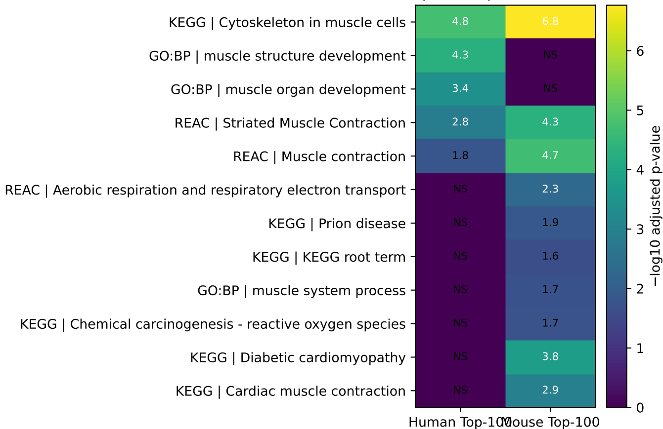
Axis B: species-specific IG enrichment
