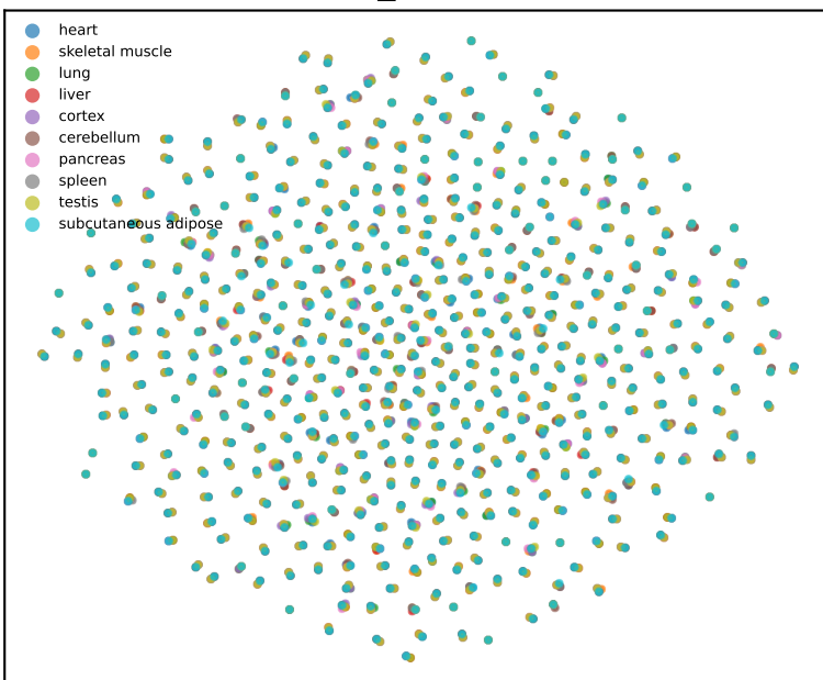
GTEx L1_early t-SNE
