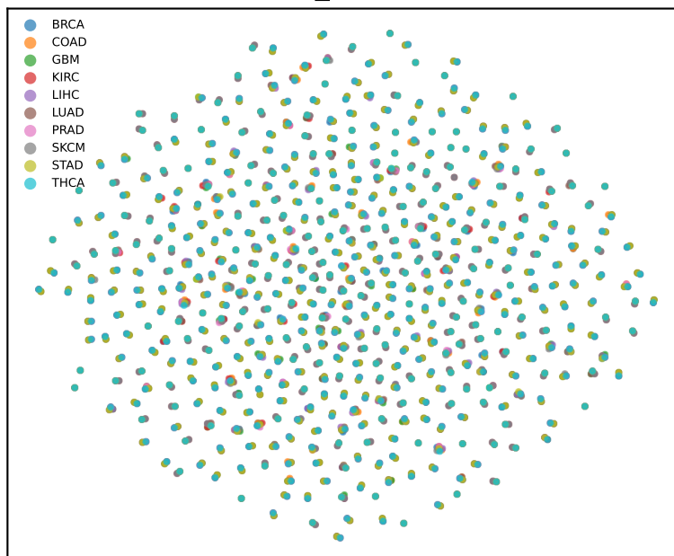
TCGA L1_early t-SNE
