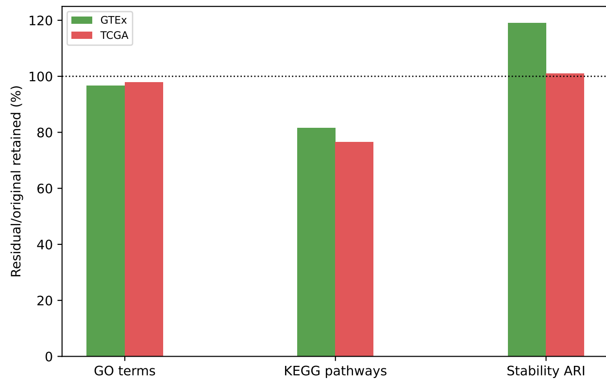
D Functional modules after linear TPM removal
