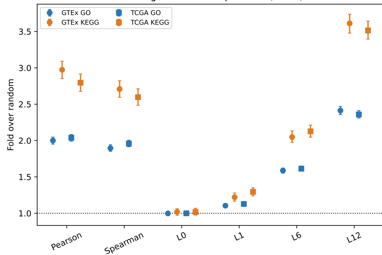
D Functional modules after linear TPM removal
