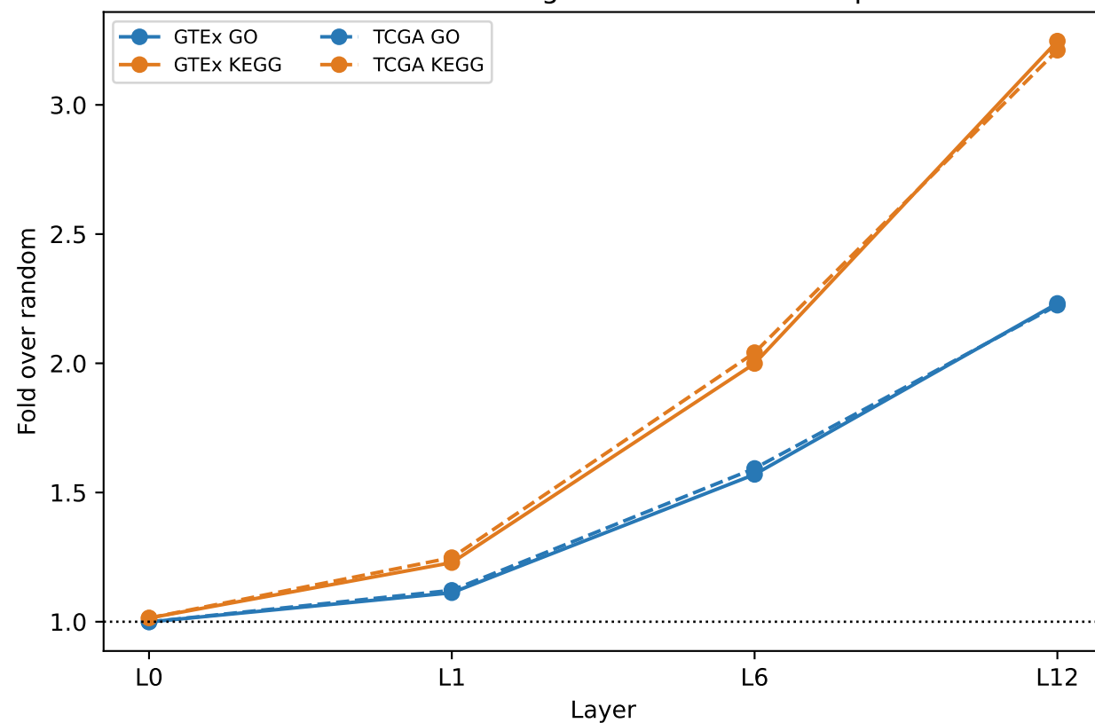
C L12 contribution after expression controls
