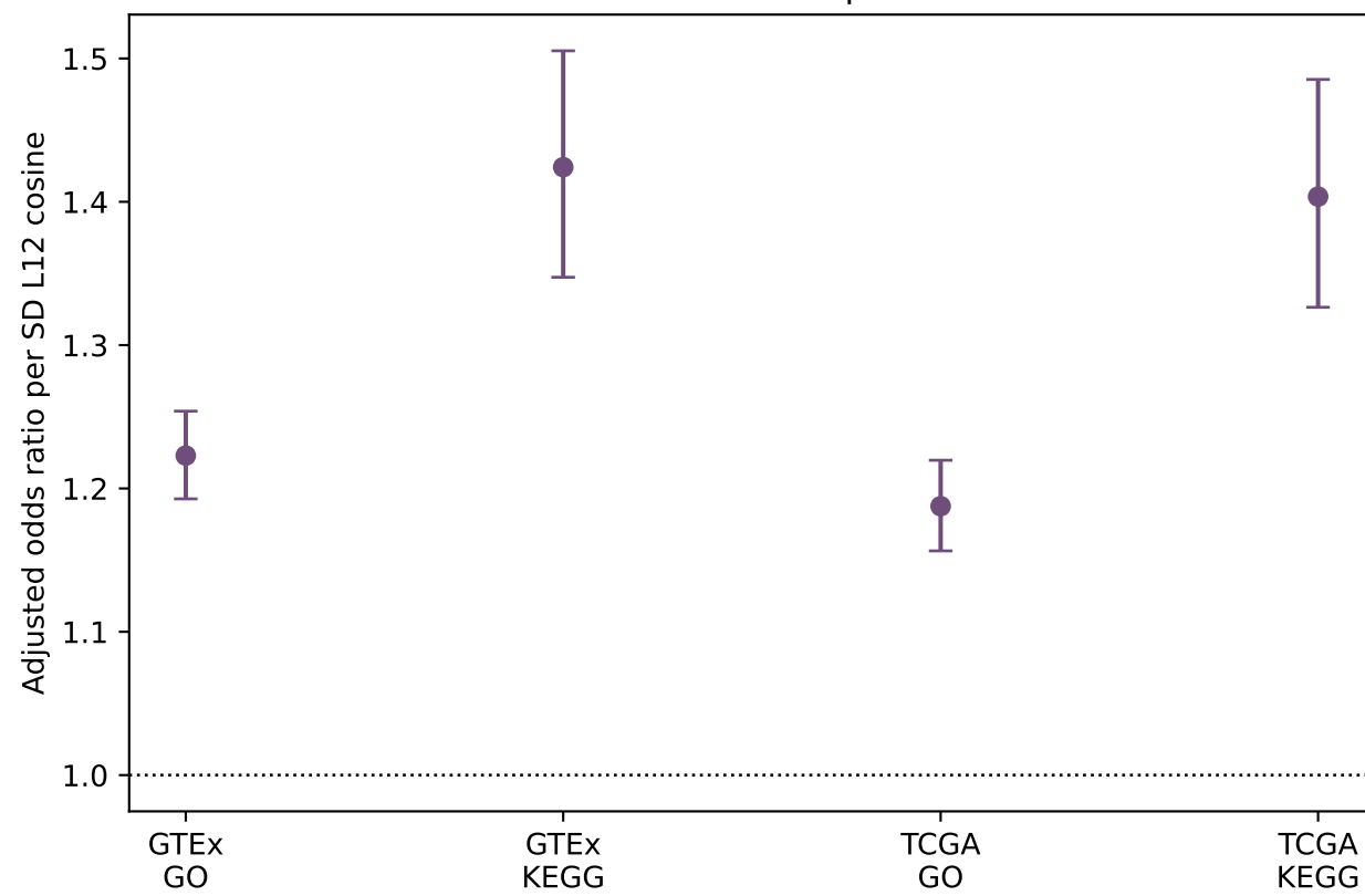
C L12 contribution after expression controls
