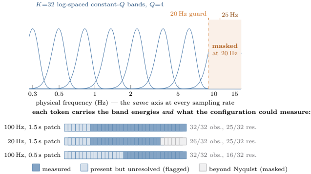
Figure 7: The filterbank, and what a token carries. Top: K=32 Gaussian bands log-spaced over 0.3–15 Hz; because a native-rate zero-padded rDFT maps bin m to mr/S , one bank reads every rate without resampling. Dashed lines mark the Nyquist guard for the two lowest corpus rates. Bottom: the real observability and resolution vectors emitted alongside the energies—part of the token, not diagnostics.
