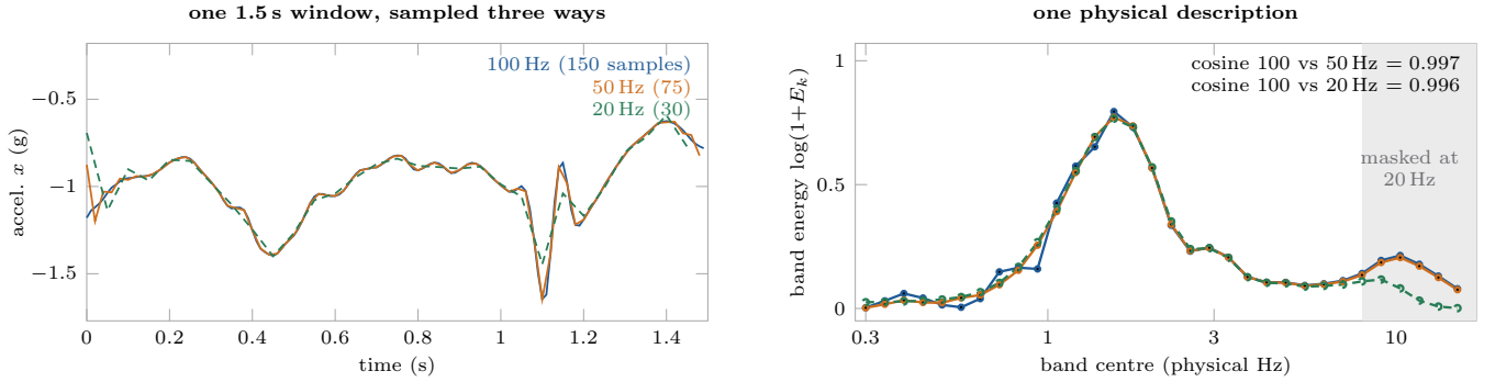
Figure 4: Rate-invariance, measured rather than argued. One 1.5 s wrist patch of walking (NFI-FARED) anti-alias resampled to three rates and run through the tokenizer at each. Left : as arrays these are three different objects—150, 75 and 30 numbers, no sample coinciding—so any encoder positioned by timestep index sees three different structures. Right : the band energies coincide (cosine 0.997 and 0.996 over the 26 commonly observable bands). The shaded region is what 20 Hz physically cannot see: those bands are masked , not estimated. The 20 Hz curve does fall away inside it—exactly the loss an encoder that resampled the whole corpus would silently take on every stream.
