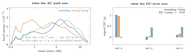
Figure 6: Why gravity is conditioned on rather than normalised away. Three static postures, UCI-HAR waist phone, 200 windows each through the real tokenizer path. Left : the frequency path receives almost nothing (note the \times 10^{-3} axis) and separates no pair distinctly—all pairwise cosines fall within 0.84–0.88. Right : signed DC places lying nearly orthogonal to standing ( -0.04 ), because gravity has redistributed across axes. The limit is shown too: standing and sitting stay at 0.99 in DC, the same pair Section 3.3 finds inseparable in text.
