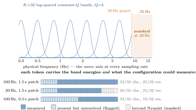
Figure 8: The filterbank, and what a token carries. Top : K=32 Gaussian bands log-spaced over 0.3–15 Hz; because a native-rate zero-padded rDFT maps bin m to mr/S , one bank reads every rate without resampling. Dashed lines mark the Nyquist guard for the two lowest corpus rates. Bottom : the real observability and resolution vectors emitted alongside the energies—part of the token, not diagnostics.
