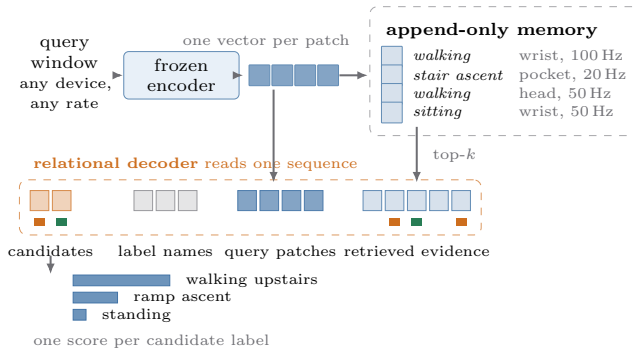
Figure 4: How a decision is made without a sensor-to-text projection. Each patch of the query retrieves independently, by cosine similarity in sensor space, from one flat memory whose rows may come from any device—that is what physical-Hz anchoring buys, and it is what a resampling or rate-conditioned encoder cannot offer without a per-configuration index. The decoder then reads a single sequence, so candidates, the label names present in the roster, the query, and the retrieved rows are all contextualised together. Which rows were enrolled for which candidate is carried by a discrete coreference slot rather than by a text similarity—the one place the geometry of Section 3.3 would otherwise re-enter. Label text is used only to name what a neighbour was and to enumerate what the deployment will accept as an answer, never as a metric. Structural diagram—the bar lengths are illustrative, not measured.
