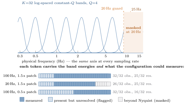
Figure 8: The filterbank, and what a token carries. Top : K=32 Gaussian bands log-spaced over 0.3–15 Hz; because a native-rate zero-padded rDFT maps bin m to mr/S , one bank reads every rate without resampling. Dashed lines mark the Nyquist guard for the two lowest corpus rates. Bottom : the real observability and resolution vectors emitted alongside the energies—part of the token, not diagnostics.
