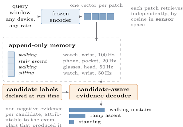
Figure 4: How a decision is made without a sensor-to-text projection. Each patch of the query retrieves independently, by cosine similarity in sensor space, from one flat memory whose rows may come from any device—that is what physical-Hz anchoring buys, and it is what a resampling or rate-conditioned encoder cannot offer without a per-configuration index. Label text enters only twice, and never as a metric: to name what a neighbour was, and to enumerate what the deployment will accept as an answer. The decoder emits non-negative evidence per candidate, attributable to the exemplars that produced it. Structural diagram—the bar lengths are illustrative, not measured.
