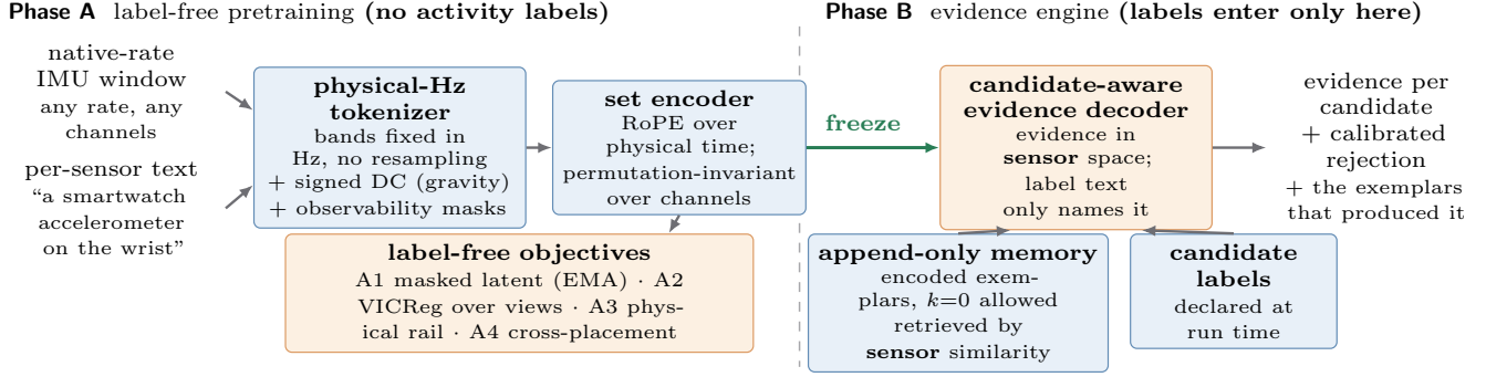
Figure 3: HALO end to end. One left-to-right path. Phase A trains the tokenizer and encoder with objectives that never see an activity label. The encoder is then frozen and crosses the boundary unchanged—it is the same weights that encode a query and that encoded every exemplar in memory, which is what lets the two be compared as vectors. Phase B adds no parameters to that path: it appends encoded exemplars to a memory and accumulates evidence for the label strings declared at run time. Adding an activity, a placement, or a device is an append; no gradient step occurs anywhere to the right of freeze.
