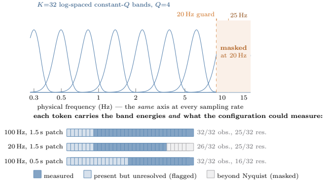
Figure 8: The filterbank, and what a token carries. Top: K=32 Gaussian bands log-spaced over 0.3–15 Hz; because a native-rate zero-padded rDFT maps bin m to mr/S , one bank reads every rate without resampling. Dashed lines mark the Nyquist guard for the two lowest corpus rates. Bottom: the real observability and resolution vectors emitted alongside the energies—part of the token, not diagnostics.
