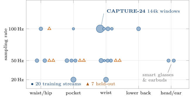
Figure 5: The corpus does not cover a grid; it covers a scatter. Each blue disc is one of the 20 sensor streams HALO trains on, positioned by body placement and native sampling rate, with area proportional to the number of 6 s windows it contributes; orange triangles are the 7 held-out evaluation datasets. Rates span a 5\times range and placements include two—smart glasses and wireless earbuds—that no established HAR benchmark contains. Held-out cells are not simply new subjects: they combine placements and rates in proportions the training corpus never sees. Absorbing this by resampling to a common rate would discard the content above 10 Hz that only the 50/100 Hz streams can resolve.
