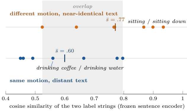
Figure 2: Sensor similarity and linguistic similarity are inverted, not merely noisy. Each dot is one pair of activity names from our label vocabulary, placed at the cosine similarity of their frozen sentence embeddings (all-MiniLM-L6-v2, the encoder language-aligned HAR models use). Pairs in the top lane denote physically distinct activities; pairs in the bottom lane denote the same physical motion. If text similarity tracked sensor similarity the lanes would separate, with the bottom lane on the right. They separate the wrong way: the mean of the physically distinct pairs (0.77) exceeds the mean of the physically identical pairs (0.60), and 38 of the 49 cross-lane comparisons are inverted. The motion grouping is our judgement; the similarities are measured. A single projection from sensor space into this text geometry is therefore mis-specified—which is why HALO retrieves in sensor space and votes in label space (Section 4.3).
