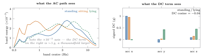
Figure 6: Why gravity is conditioned on rather than normalised away. Three static postures, UCI-HAR waist phone, 200 windows each through the real tokenizer path. Left: the frequency path receives almost nothing (note the \times 10^{-3} axis) and separates no pair distinctly—all pairwise cosines fall within 0.84–0.88. Right: signed DC places lying nearly orthogonal to standing ( -0.04 ), because gravity has redistributed across axes. The limit is shown too: standing and sitting stay at 0.99 in DC, the same pair Section 3.3 finds inseparable in text.
