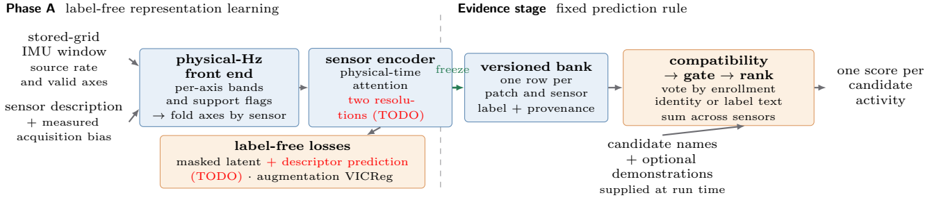
Figure 2: HALO end to end. Phase A learns one sensor representation without activity labels. A versioned bank stores frozen per-patch, per-sensor rows. Classification applies hard compatibility, candidate-conditioned admissibility, cosine ranking, voting, and sensor fusion. Enrollment appends labeled rows; it does not update parameters.
