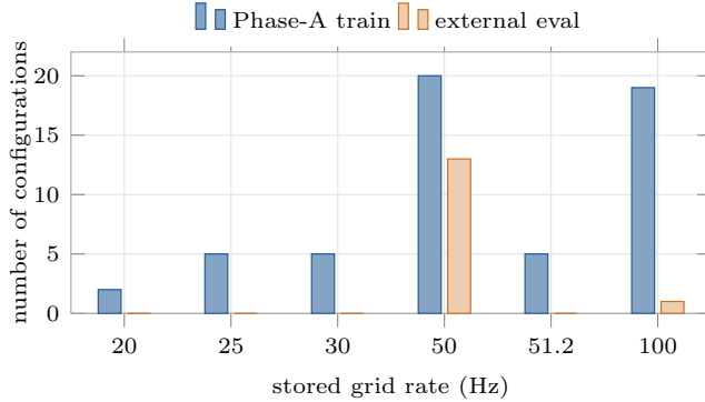
Figure 4: Materialized configurations by stored grid rate. The current roster contains 56 Phase-A configurations and 14 external-evaluation configurations. Source acquisition rate is stored separately and bounds observability when a converter has already resampled a stream.
