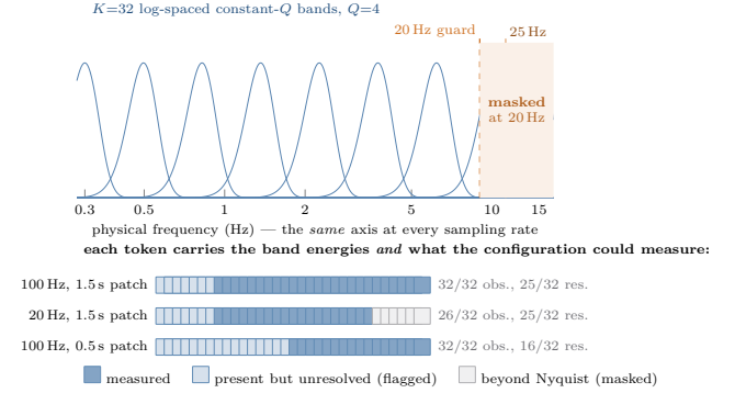
Figure 7: The filterbank, and what a token carries. Top: K=32 Gaussian bands log-spaced over 0.3–15 Hz; because a native-rate zero-padded rDFT maps bin m to mr/S , one bank reads every rate without resampling. Dashed lines mark the Nyquist guard for the two lowest corpus rates. Bottom: the real observability and resolution vectors emitted alongside the energies—part of the token, not diagnostics.
