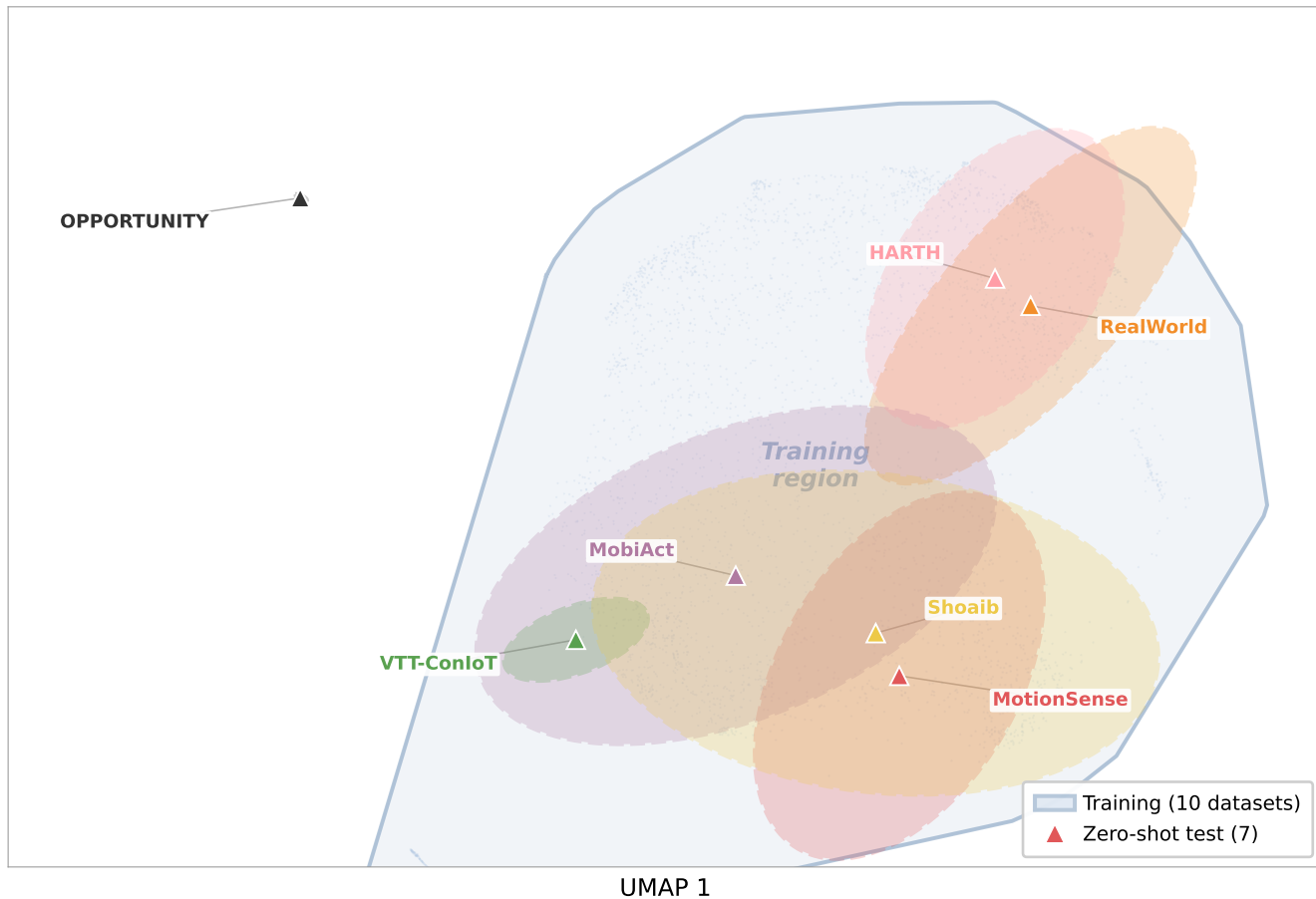
Distribution Gap Between Training and Zero-Shot Test Datasets
