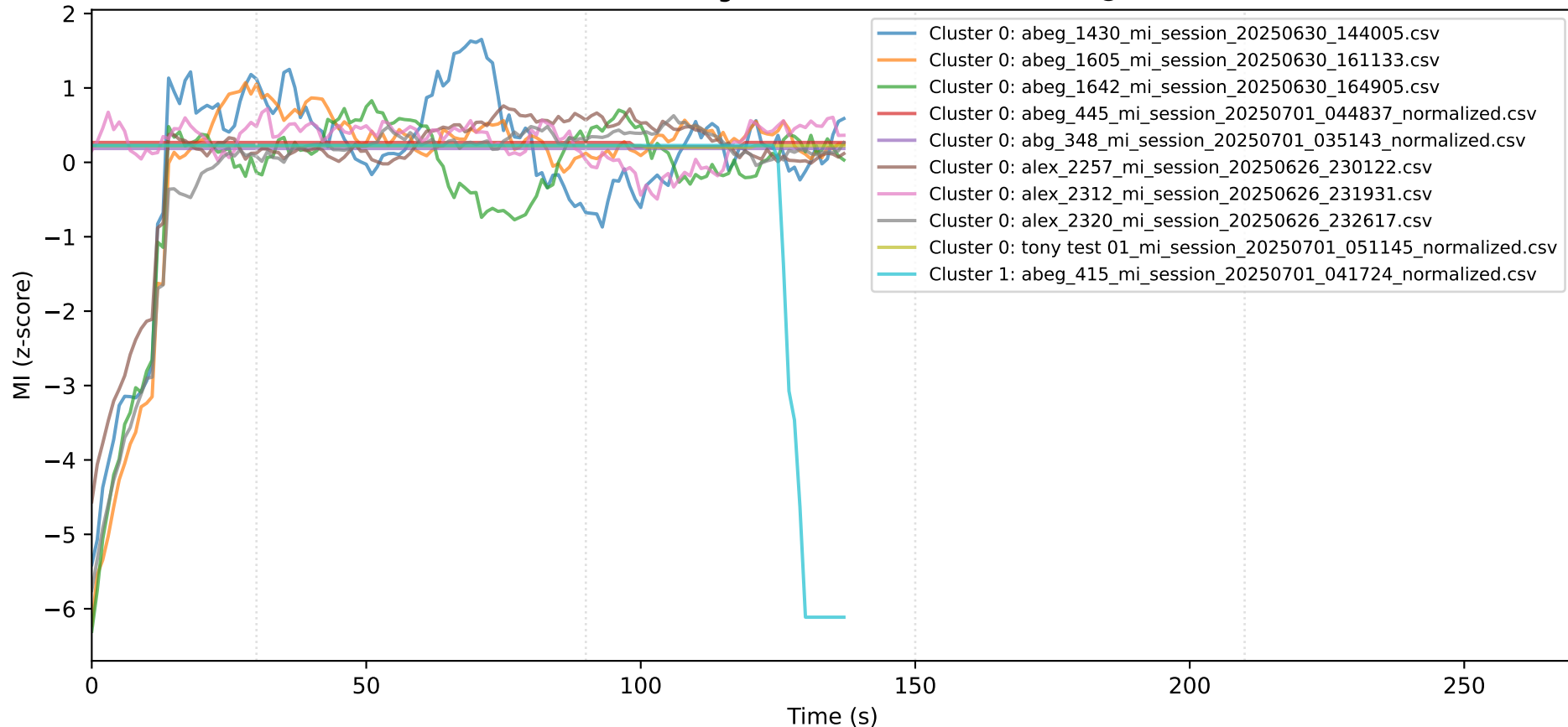
KMeans Clustering of MI Curves (k=2) - 270s @ 1Hz
