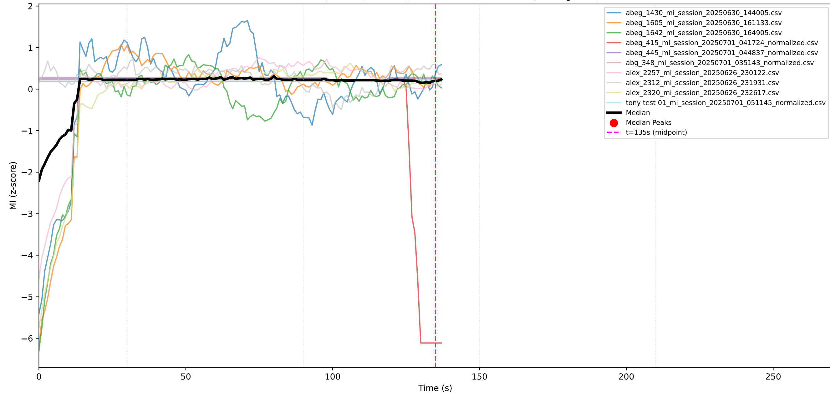
MI Curves (z-score, MA=20) with Median and Peaks (270s @ 1Hz)
