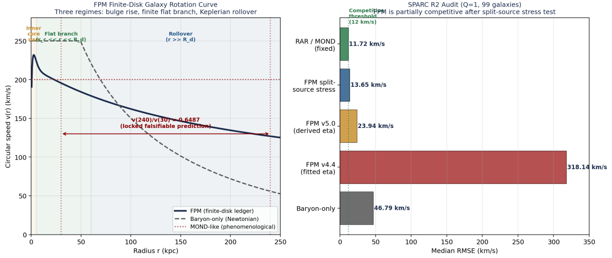
Figure 8. Left: FPM finite-disk galaxy rotation curve with three regimes and the locked falsifiable prediction v(240)/v(30) = 0.6487 . Right: SPARC R2 audit showing FPM is partially competitive after split-source stress test but not a baseline victory.
