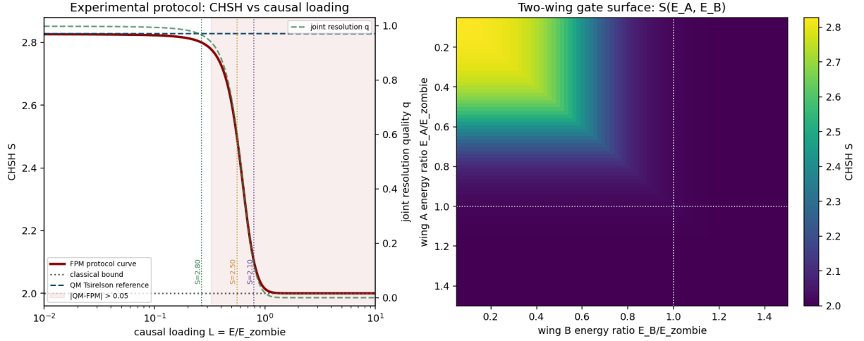
Figure 11. Proposed ZOMBIE-gated Bell signature as a causal-loading protocol. Left: CHSH is plotted against L = E/E_{\text{zombie}} with threshold markers and the region where the FPM curve diverges from a flat standard-QM Tsirelson reference. Right: the two-wing surface shows that one FLOW wing suppresses the joint violation.
