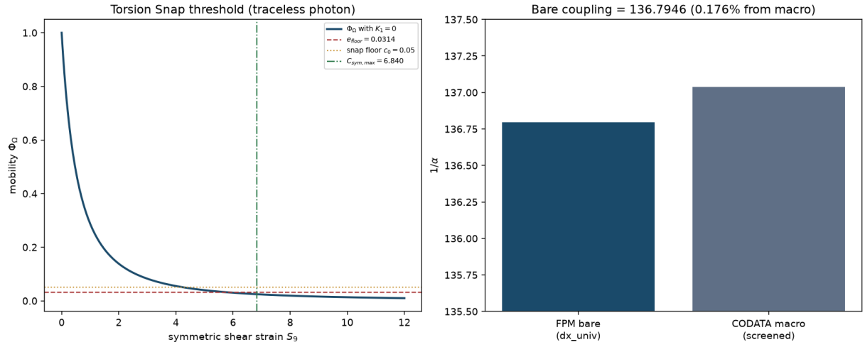
Figure 12. Fine-structure bare coupling audit. Left: traceless mobility collapse at e_{\text{floor}} defines C_{\text{sym}, \text{max}} . Right: bare grid coupling 1/136.795 vs macroscopic CODATA 1/137.036 .
