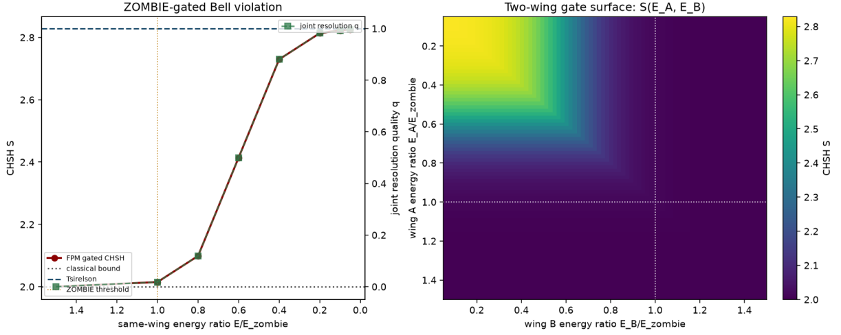
Figure 11. Proposed ZOMBIE-gated Bell signature. Left: CHSH rises from the classical bound toward Tsirelson only as both linked daemons enter deep ZOMBIE mode. Right: the two-wing surface shows that one FLOW wing suppresses the joint violation.
