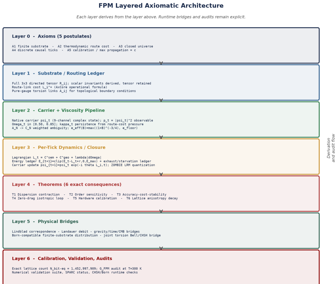
Figure 2. The layered architecture. Axioms (Layer 0) generate the routing substrate (Layer 1), the carrier and viscosity pipeline (Layer 2), per-tick closure dynamics (Layer 3), six theorems (Layer 4), physical bridges (Layer 5), and calibration/validation audits (Layer 6).
