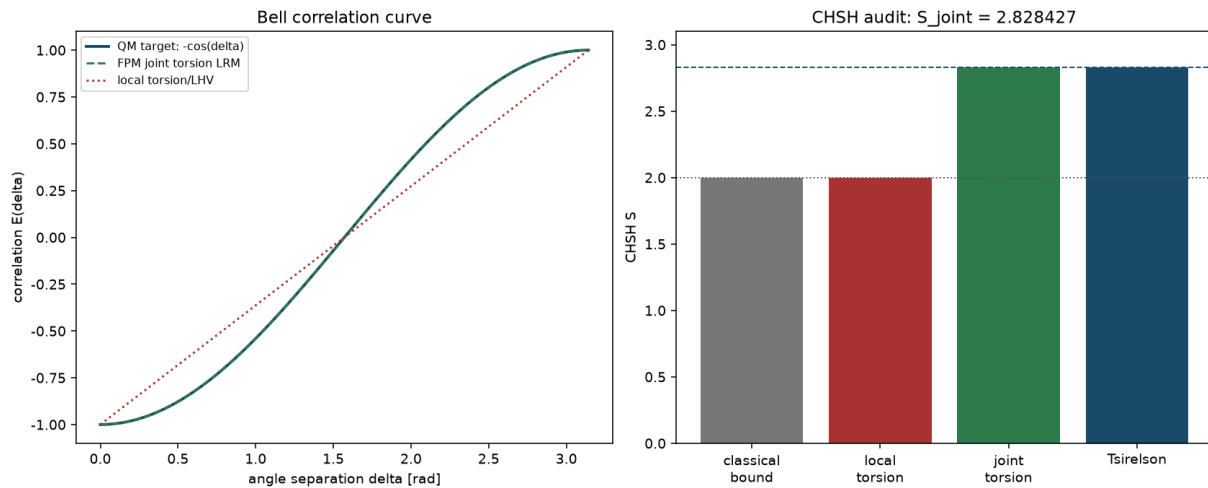
Figure 10. v5.6 Bell/CHSH audit. Left: local torsion quantization is Bell-classical, while joint torsion LRM tracks the singlet cosine correlation. Right: the joint torsion bridge reaches the Tsirelson bound S = 2.828427 .
