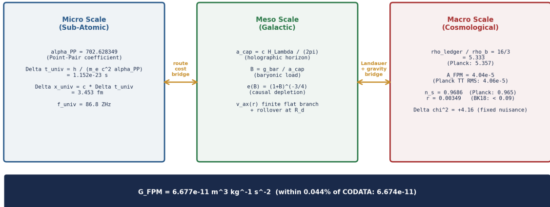
Figure 10. The calibration bridge: from sub-atomic tick (micro) through galactic dynamics (meso) to CMB horizon (macro).
