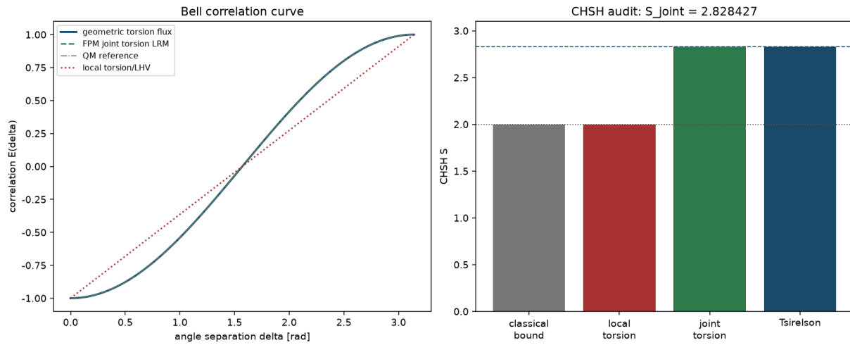
Figure 10. v5.6 Bell/CHSH audit. Left: local torsion quantization is Bell-classical, while rotated torsion flux generates the cosine correlation before LRM quantization. Right: the joint torsion bridge reaches the Tsirelson bound S = 2.828427 .
